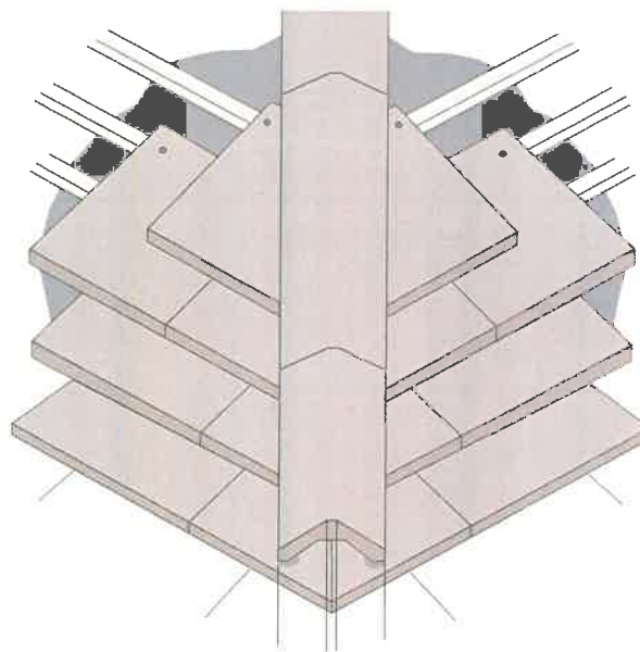
Capped hip
