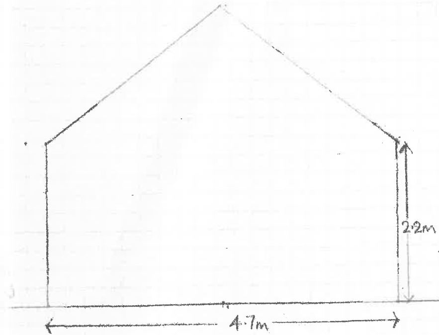
Elevation NW
