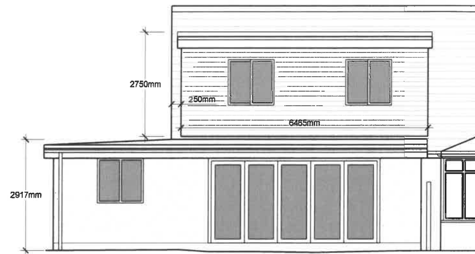
Rear Elevation
