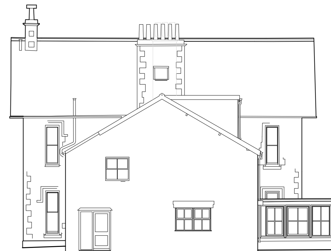
Side Elevation
