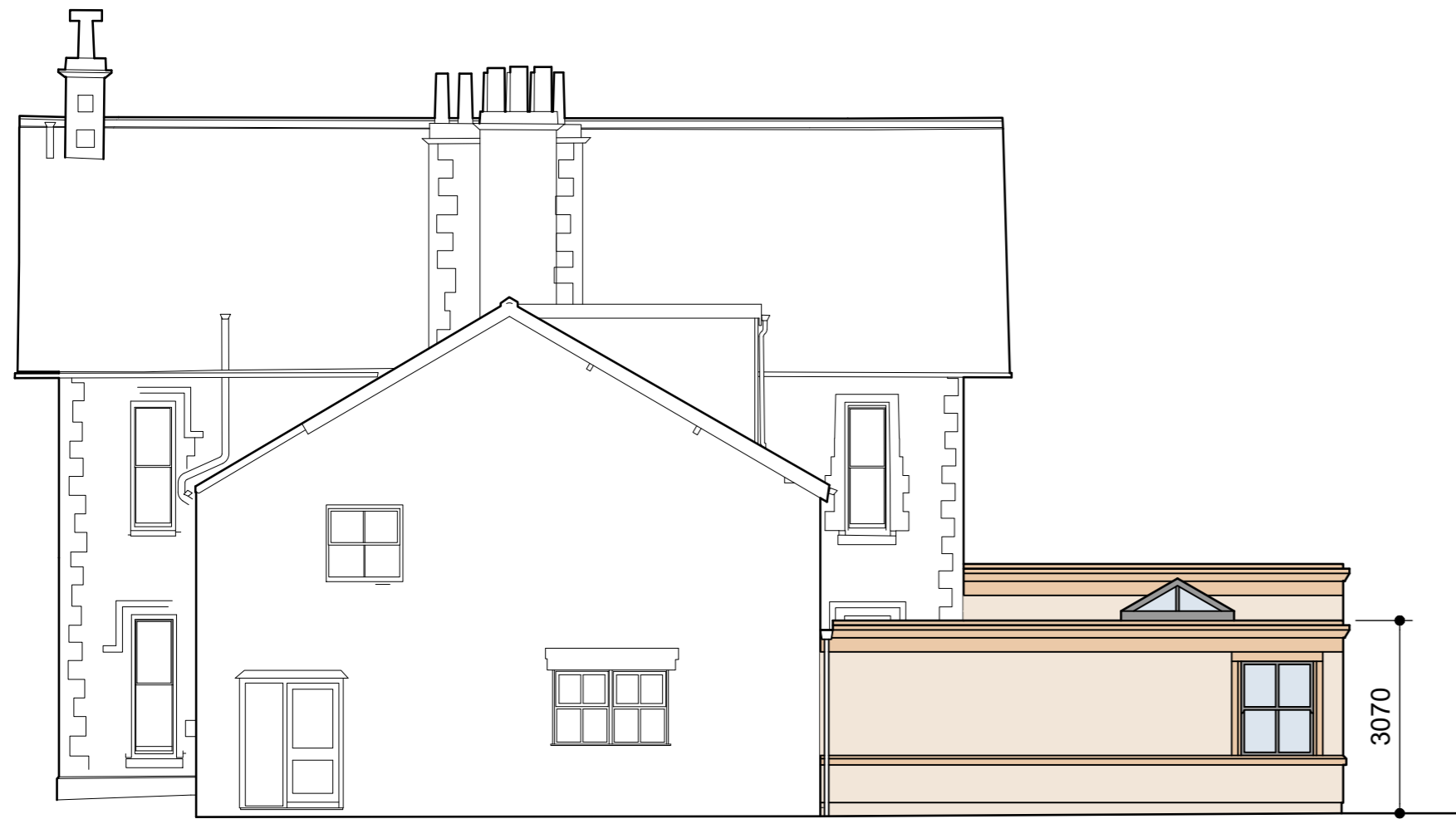
Side Elevation
