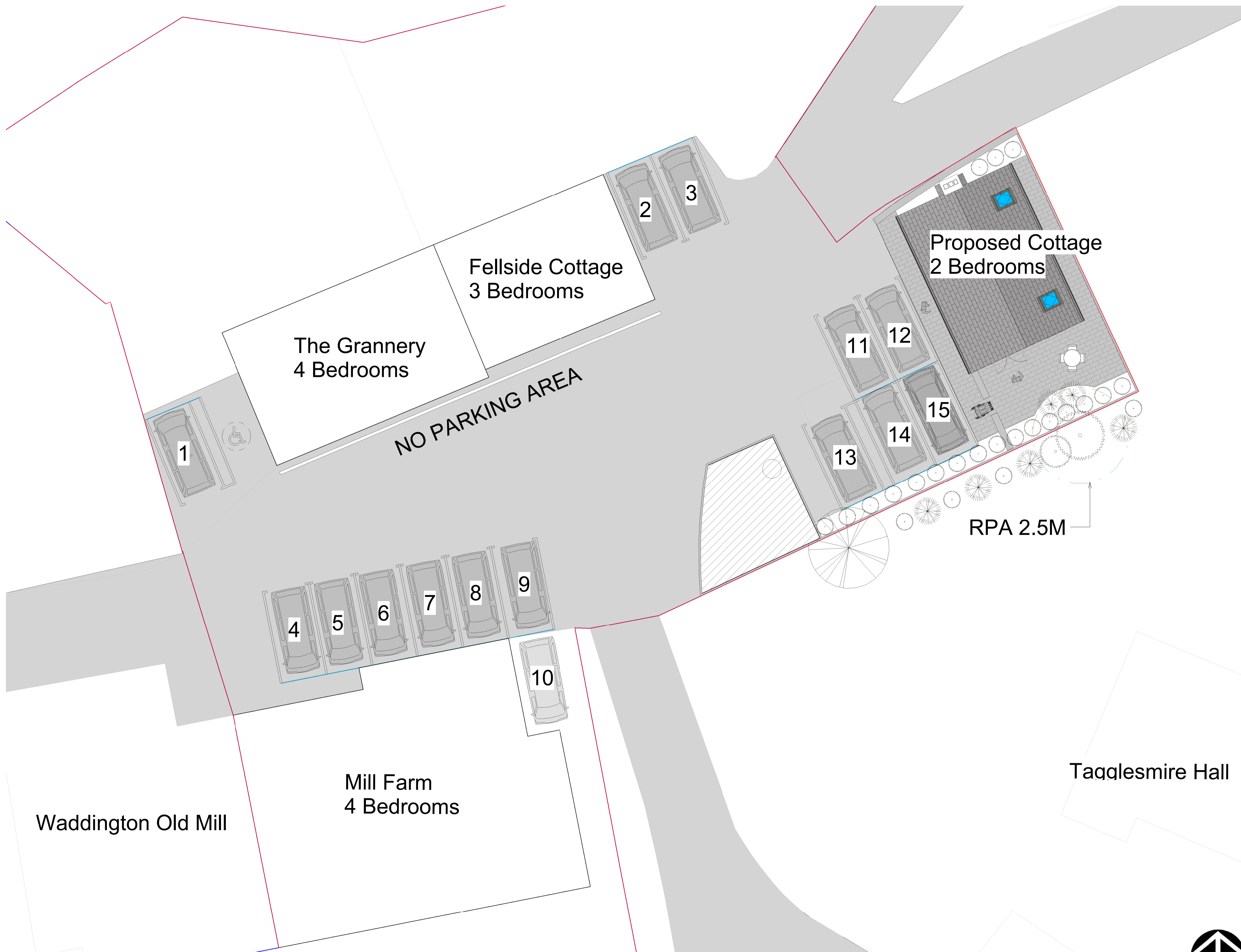
1 PROPOSED PARKING PLAN 1:100
