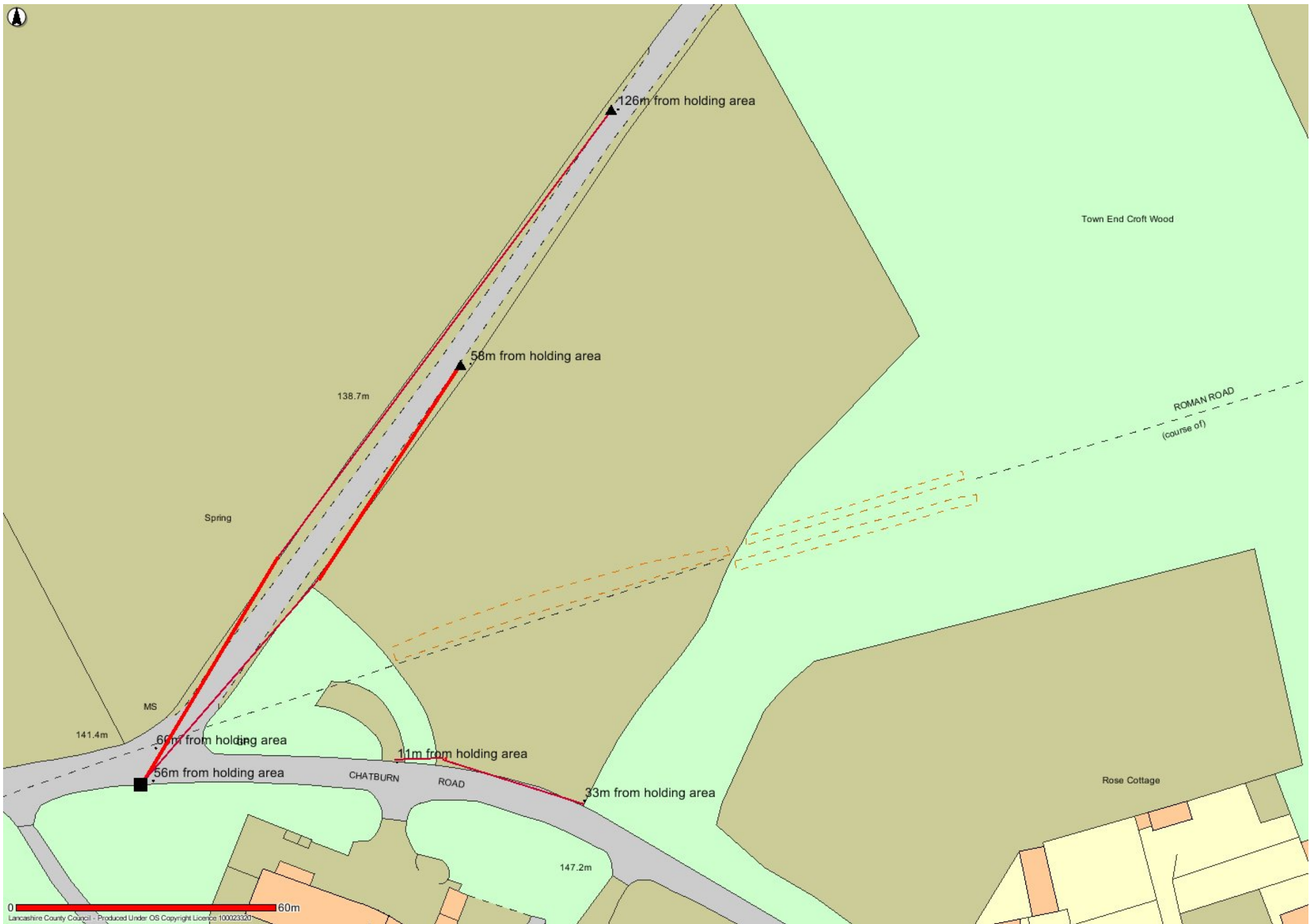
Proposed Downham Concessionary Bridleway visibility splays
