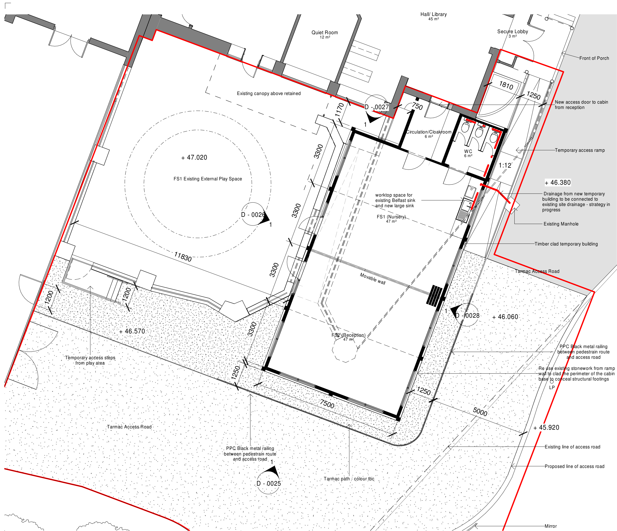
1 Proposed Ground Floor Plan - Temporary Classroom Block 1 : 100
