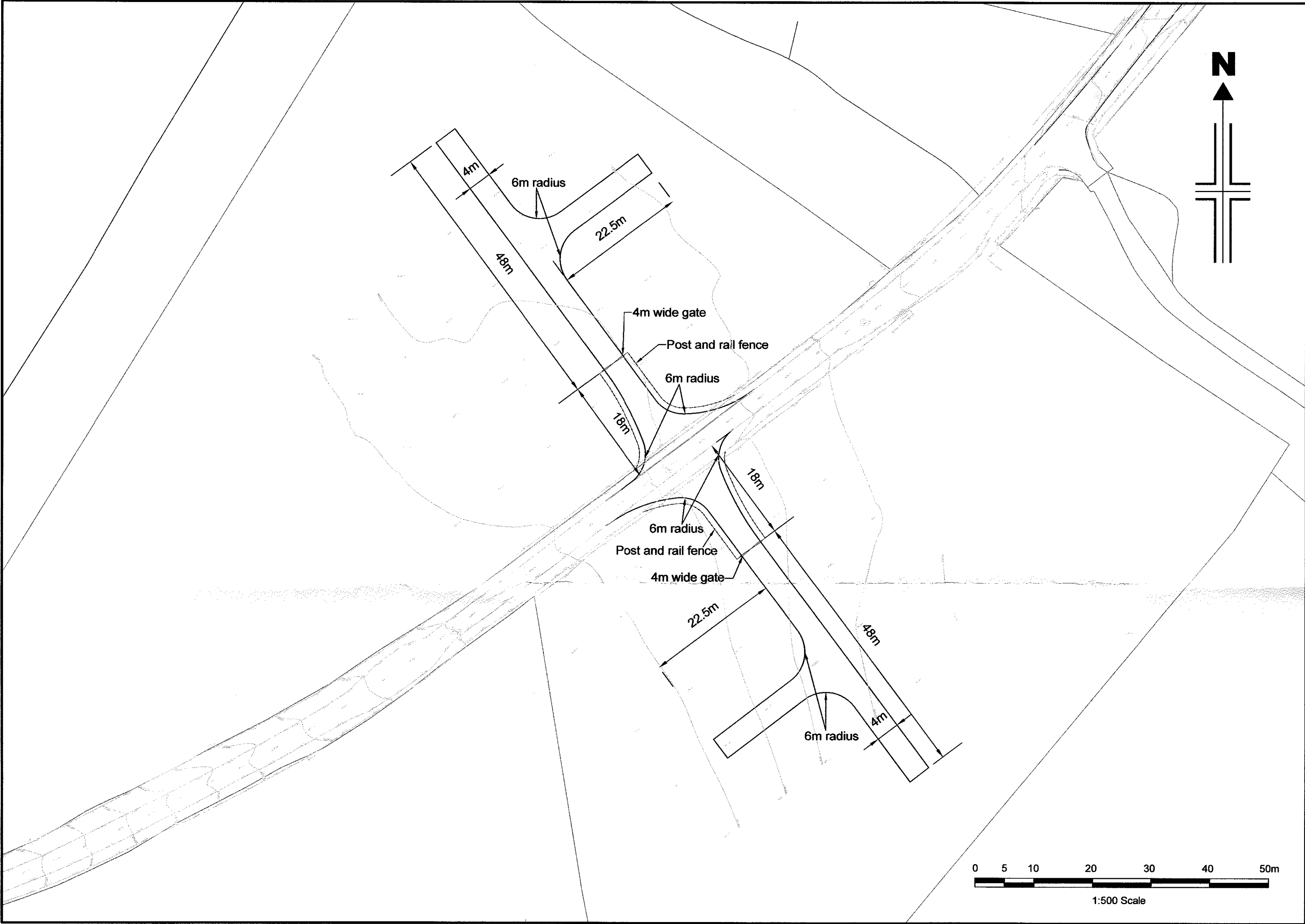
Proposed Access Track (Scale 1:500)
