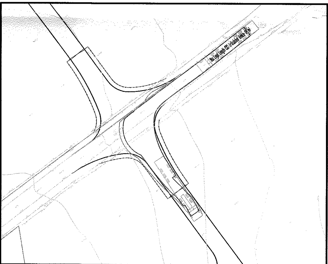
Swept Path Analysis (Max Articulated) (Scale 1:500)
