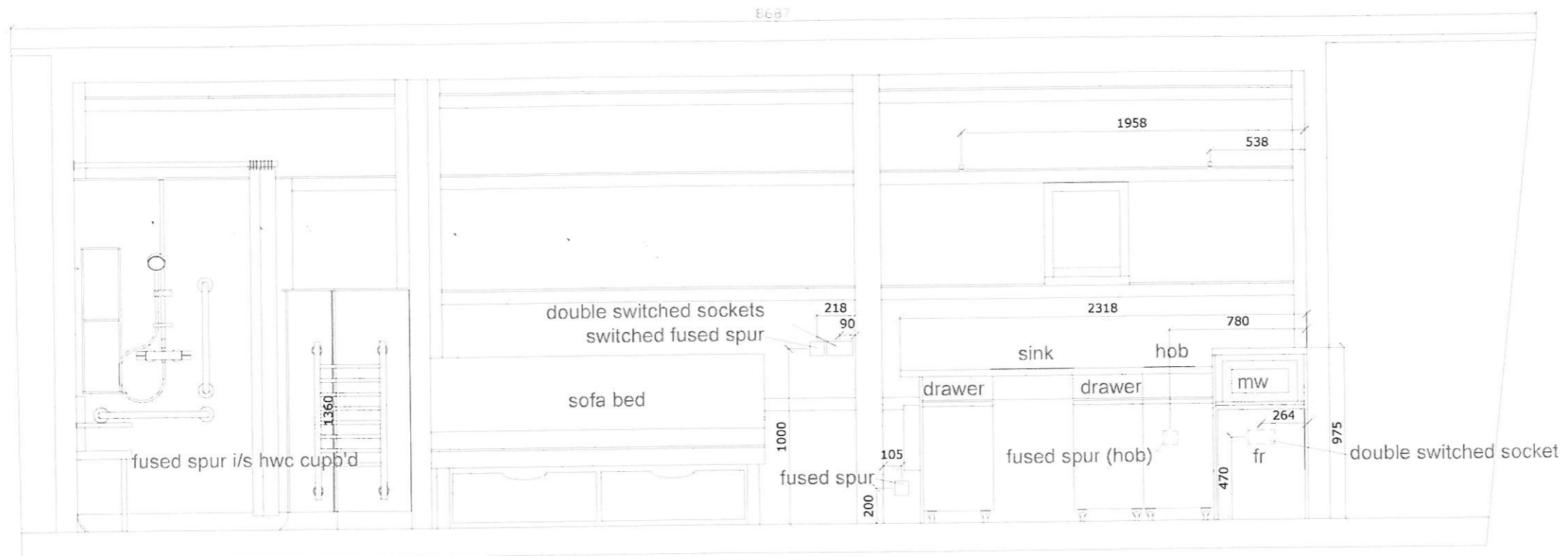
Standard Accessible Wigwam Kitchen Unit Wall
