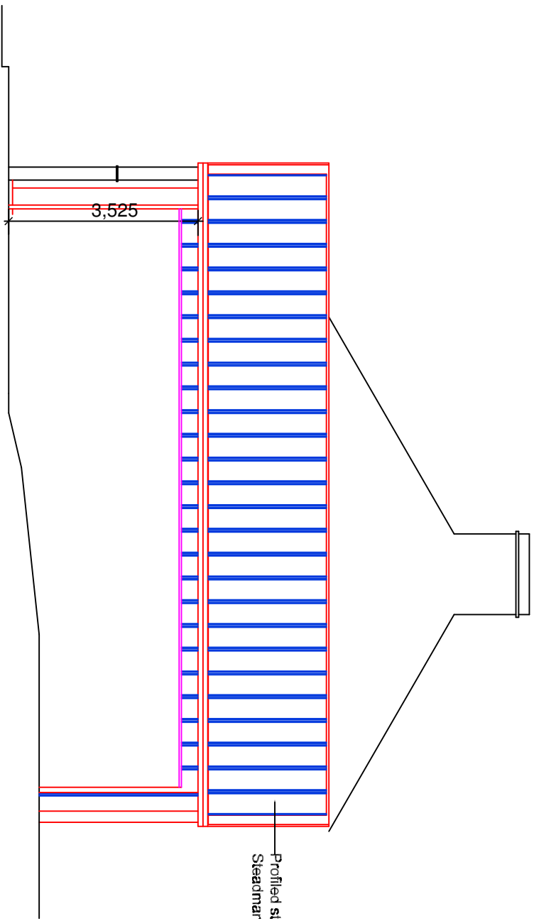
SIDE ELEVATION AS PROPOSED
