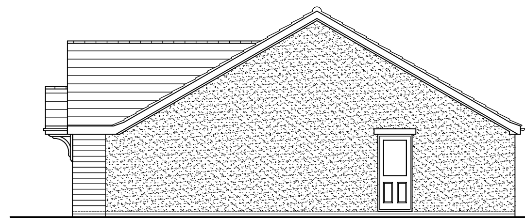
SIDE ELEVATION - RENDER 1:100
