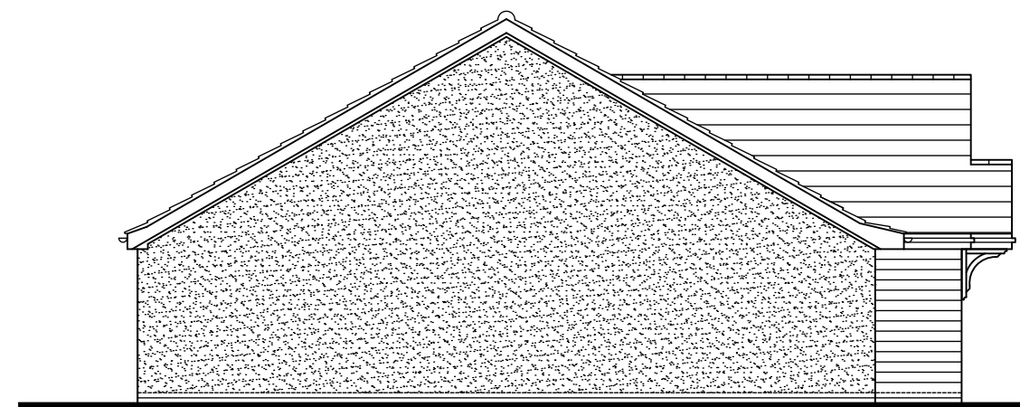
SIDE ELEVATION - RENDER 1:100
