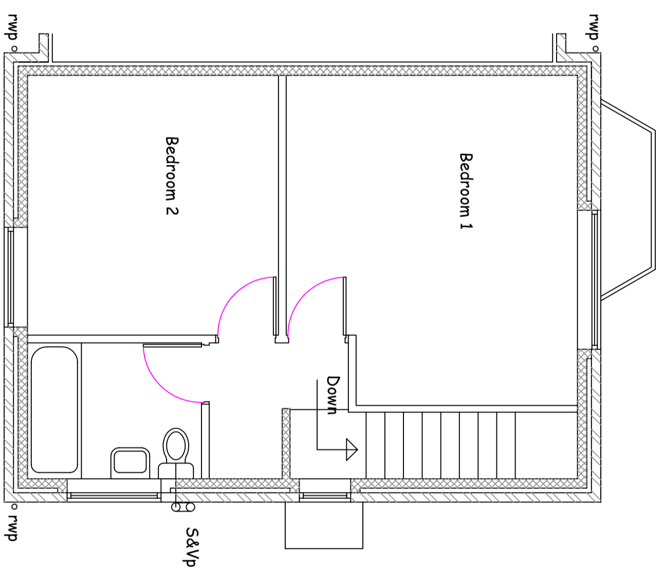
Ex First Floor
