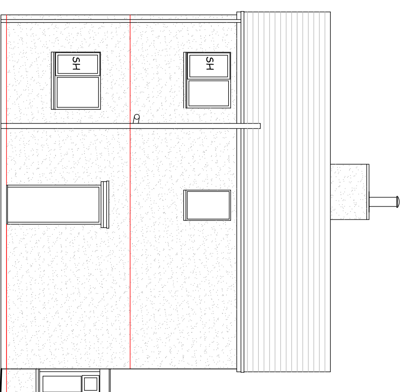
Ex Side Elevation
