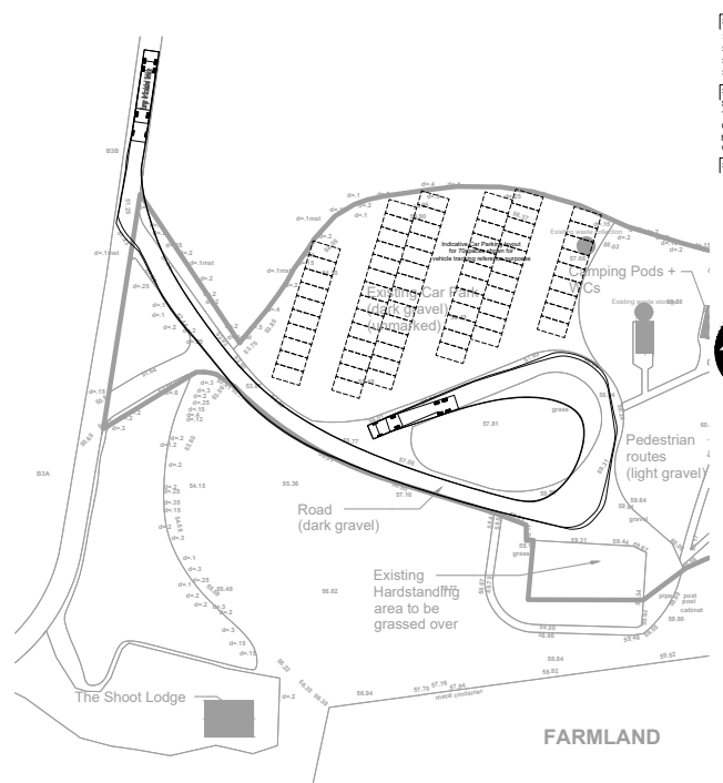
SWEPT PATH ANALYSIS FOR 15.4m LONG ARTICULATED VEHICLE - IN MANOEUVRE
