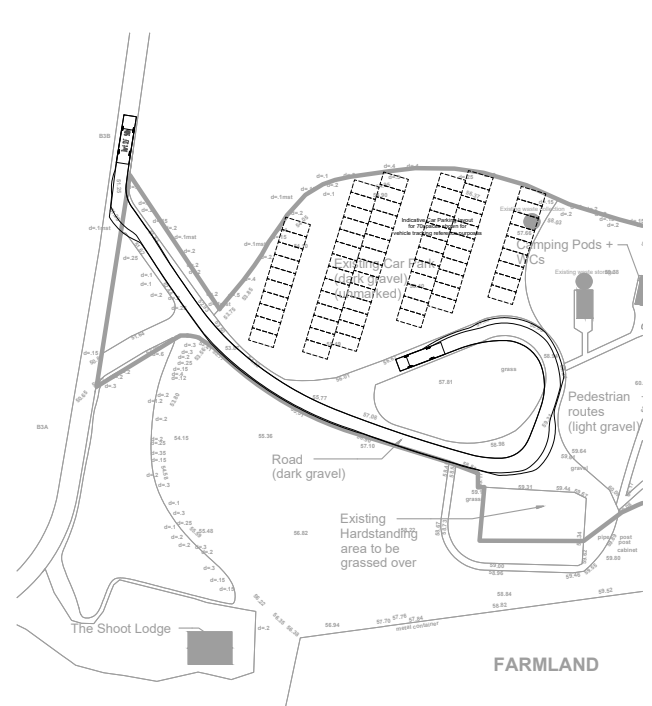
SWEPT PATH ANALYSIS FOR 9m LONG COACH - IN MANOEUVRE
