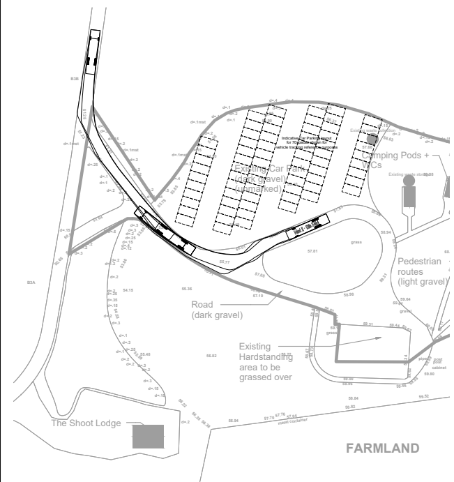
SWEPT PATH ANALYSIS FOR 12m LONG COACH - OUT MANOEUVRE
