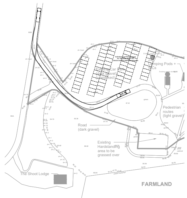
SWEPT PATH ANALYSIS FOR 9m LONG COACH - OUT MANOEUVRE
