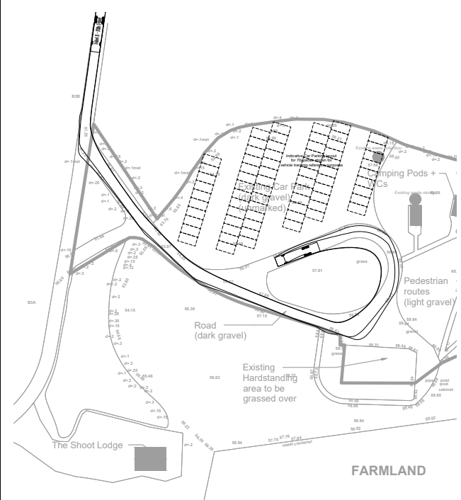
SWEPT PATH ANALYSIS FOR 12m LONG COACH - IN MANOEUVRE
