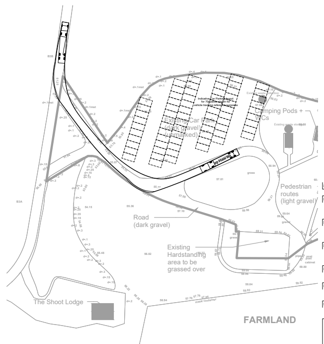
SWEPT PATH ANALYSIS FOR 15.4m LONG ARTICULATED VEHICLE - OUT MANOEUVRE
