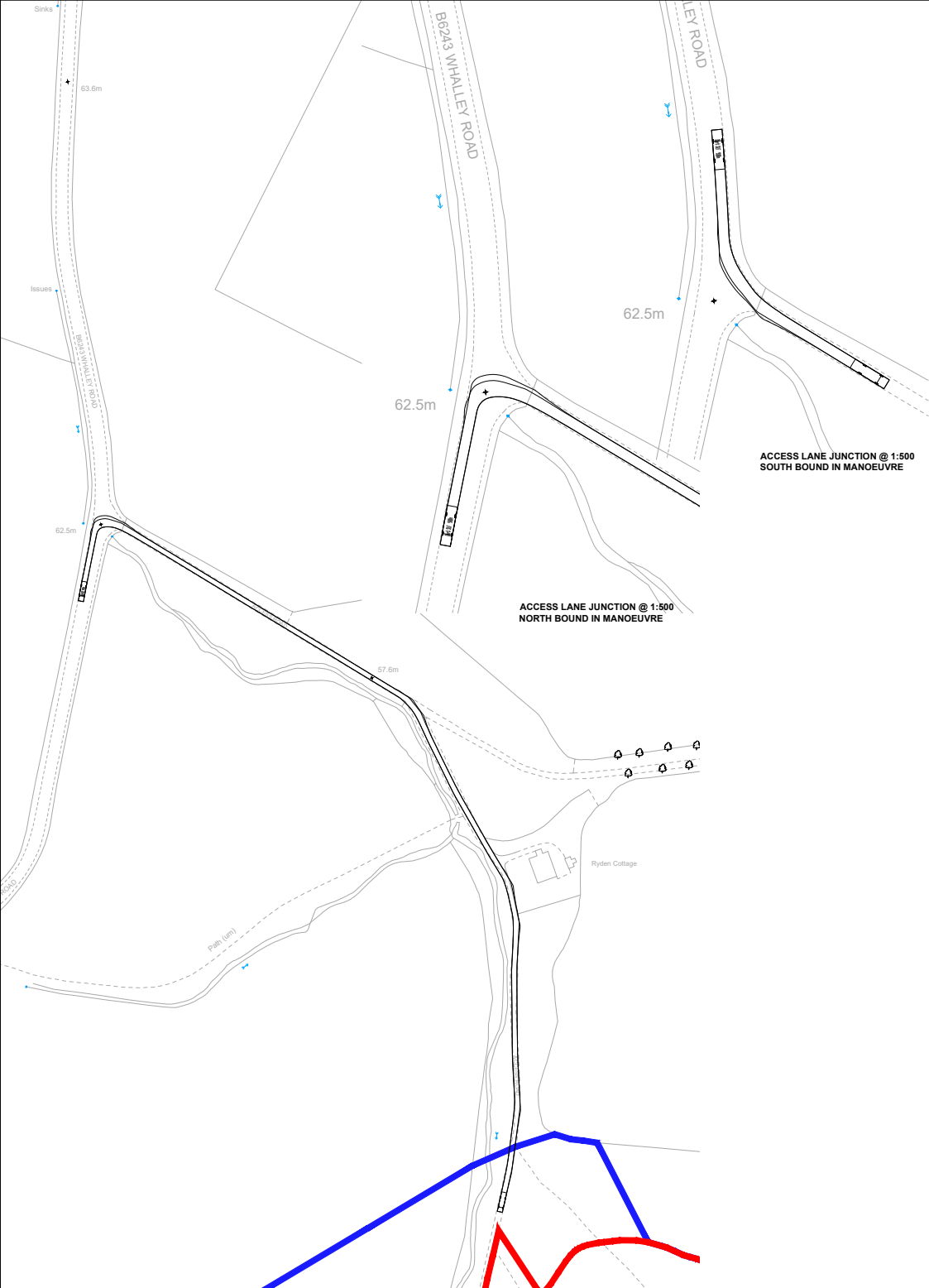
SWEPT PATH ANALYSIS FOR 9m LONG COACH - NORTH BOUND IN MANOEUVRE 1:1000
