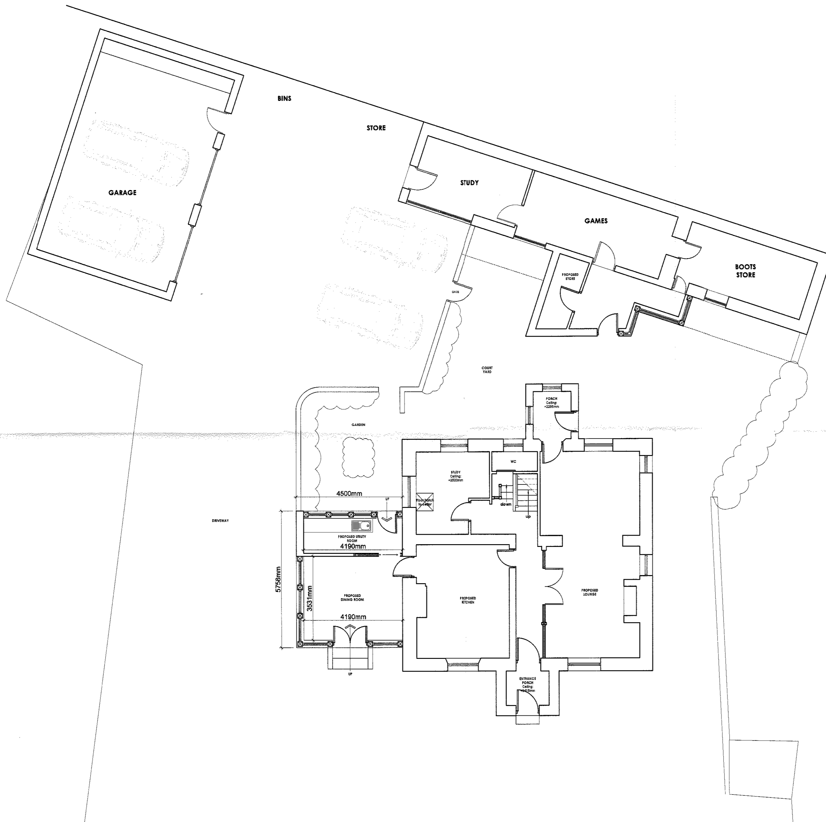
PROPOSED SITE PLAN Scale 1:100
