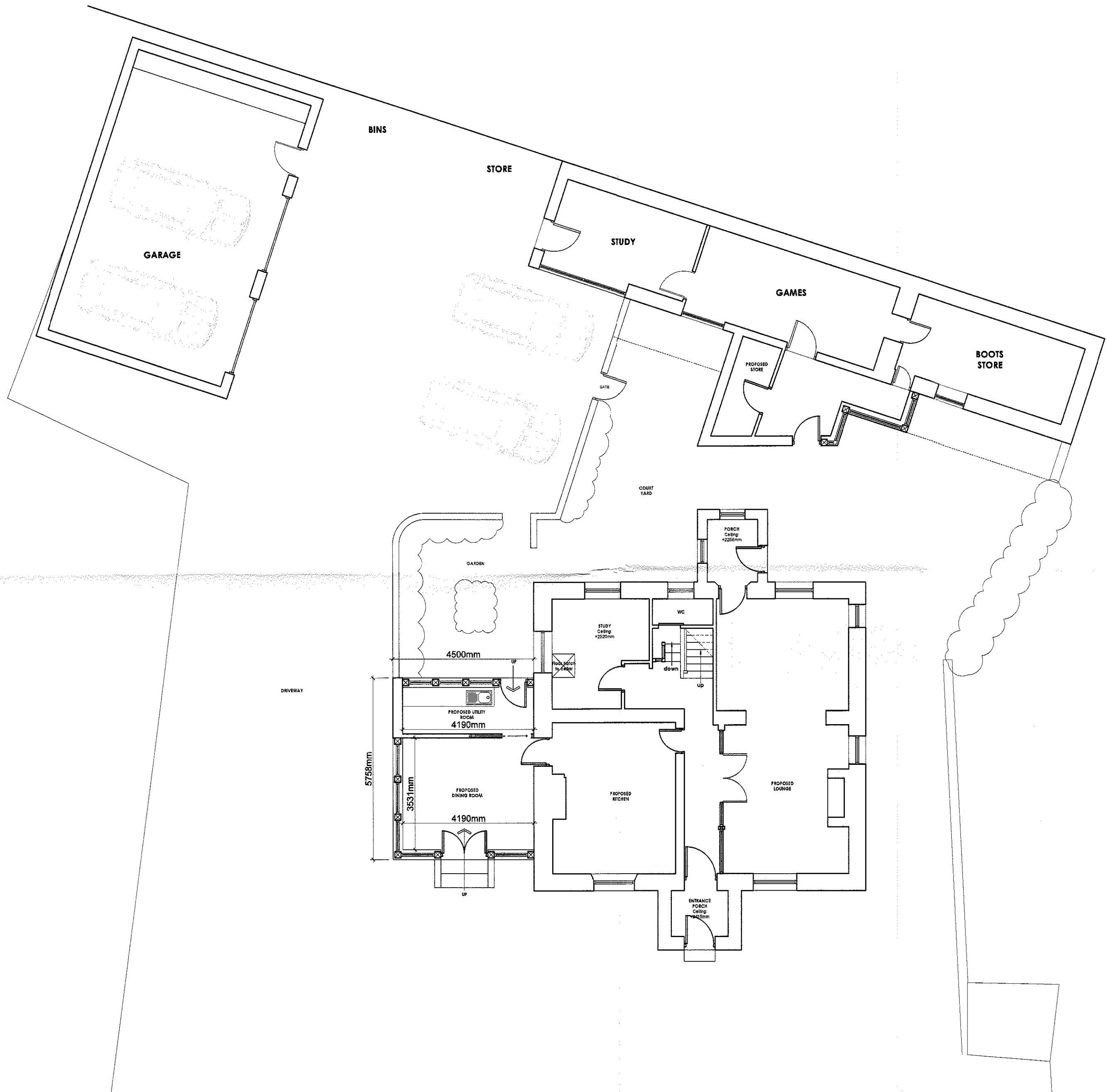
PROPOSED SITE PLAN Scale 1:100 0 2 4 6m
