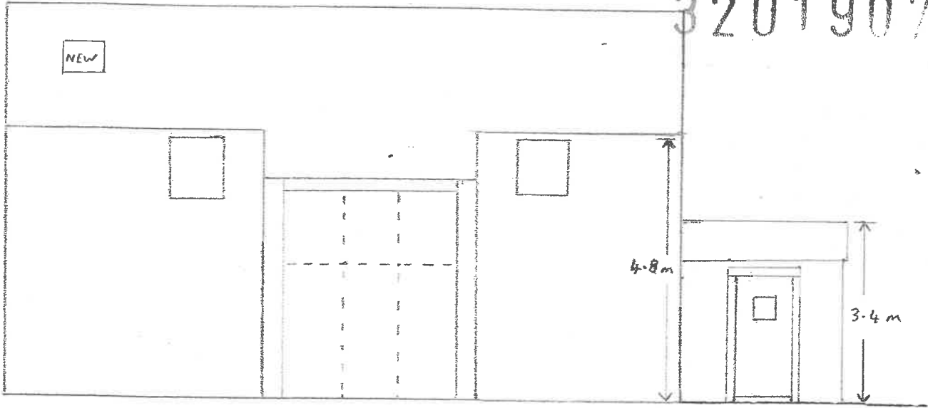
North East Front Elevation
