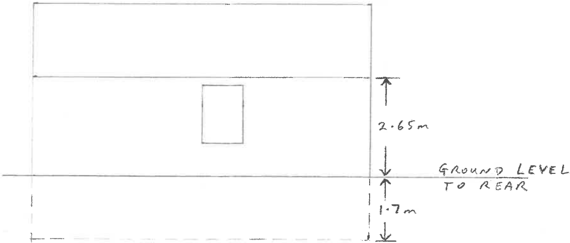
North West (to yard) Elevation
