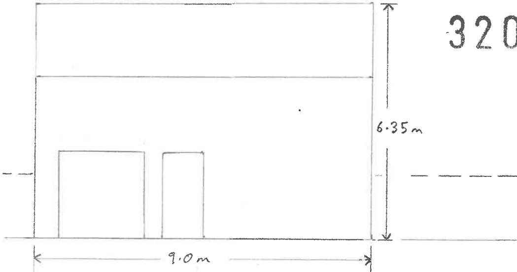
South East (to garden) Elevation
