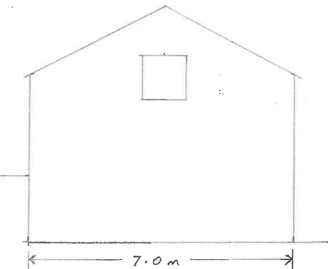
South West Gable (rear) Elevation
