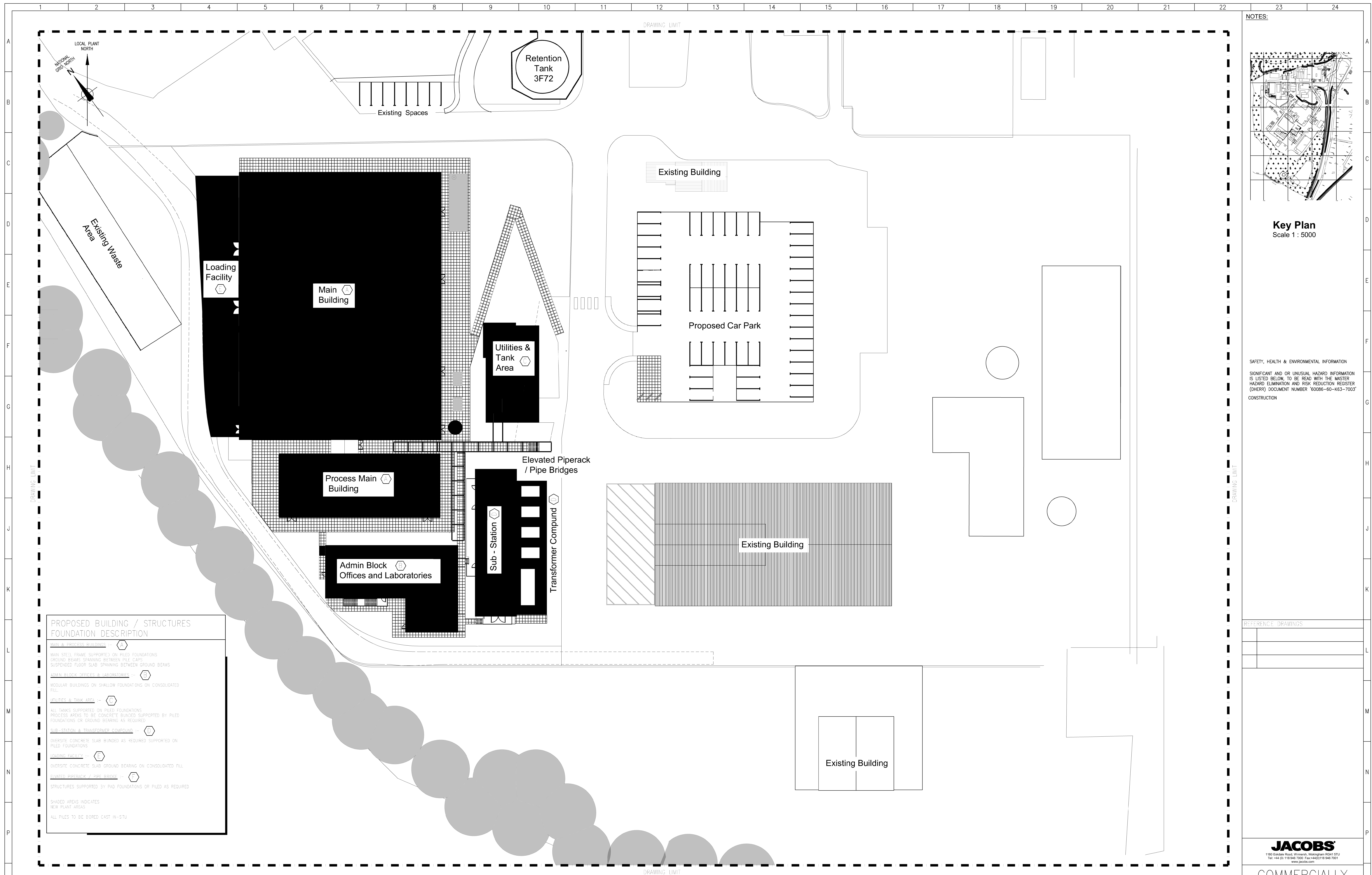
Layout Proposed Bulidings / Structures Scale 1 : 250
