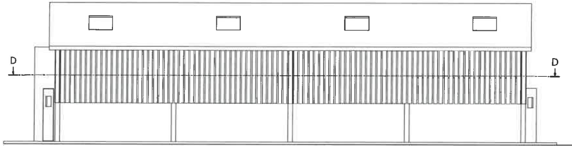
VIEW ON SIDE ELEVATION
