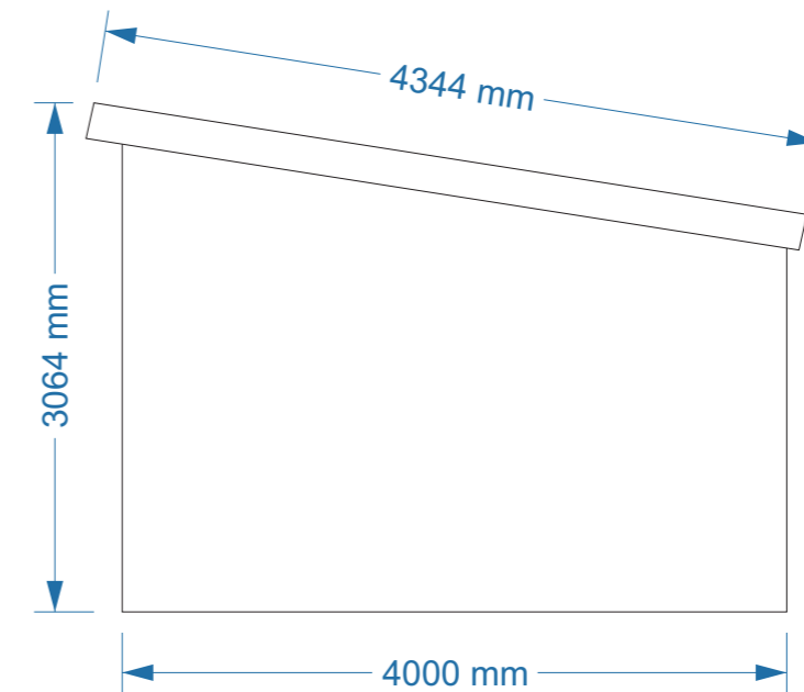
back elevation
