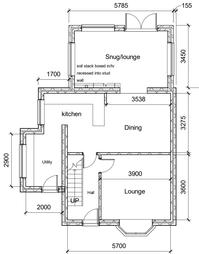
1 Ground floor 1 : 100
