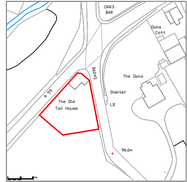
Location plan 1:1250
