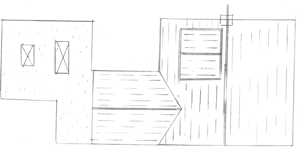
ROOF PLAN – PROPOSED SCALE 1:100
