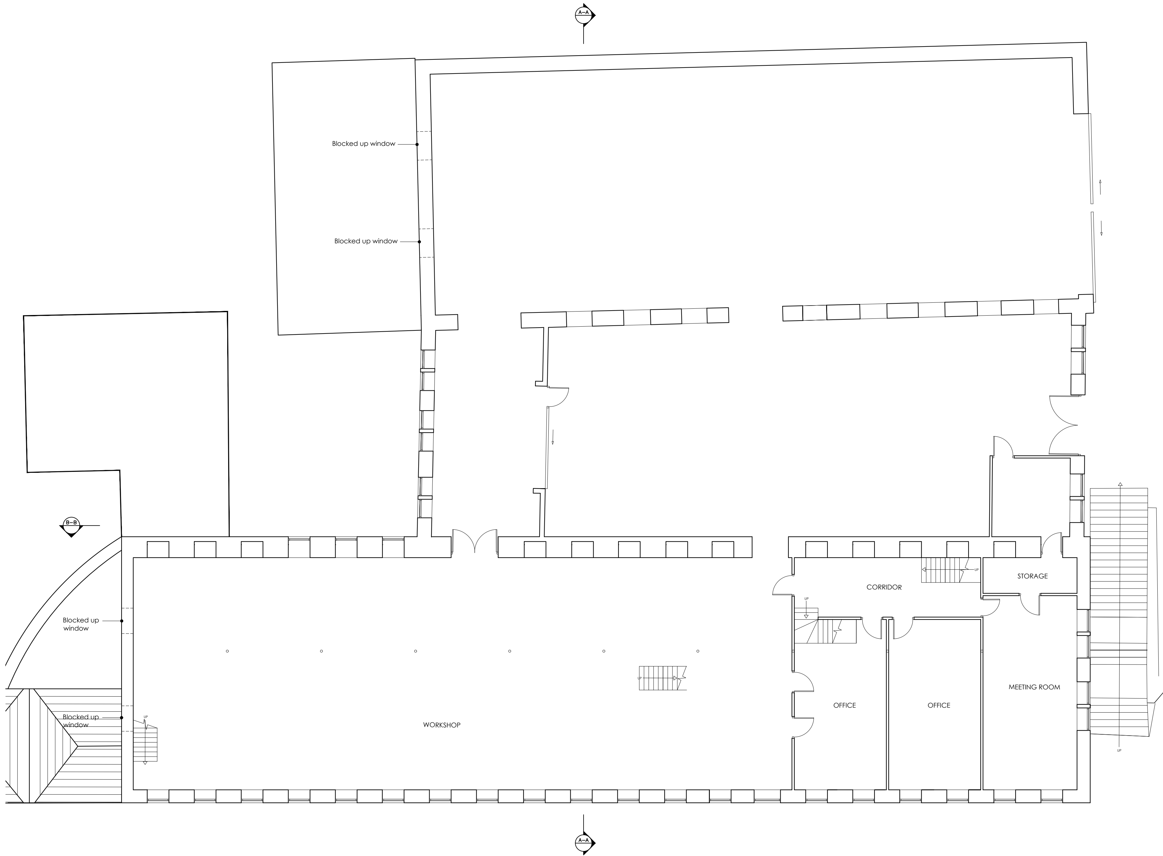
EXISTING GROUND FLOOR FLOOR PLAN SCALE 1:100
