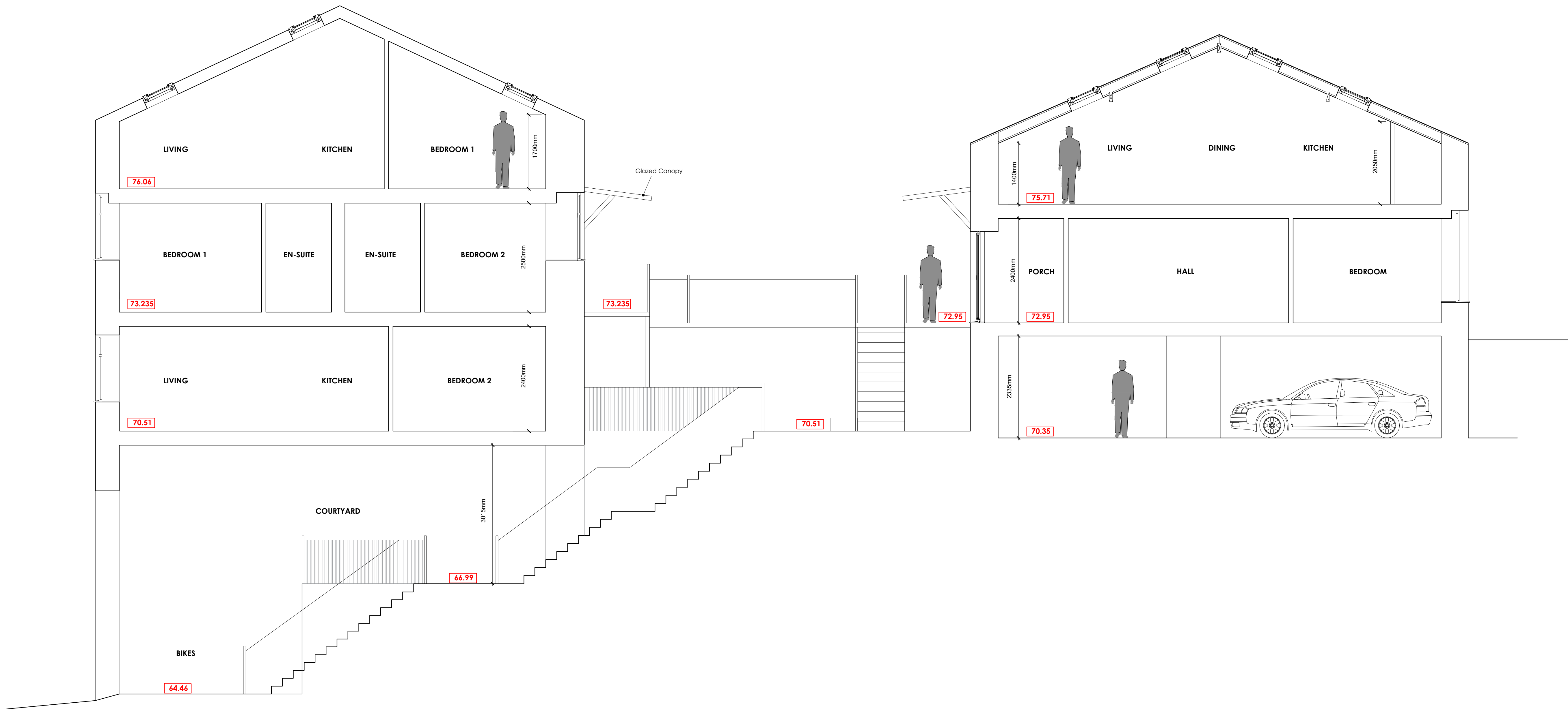
PROPOSED SECTION A-A SCALE 1:50
