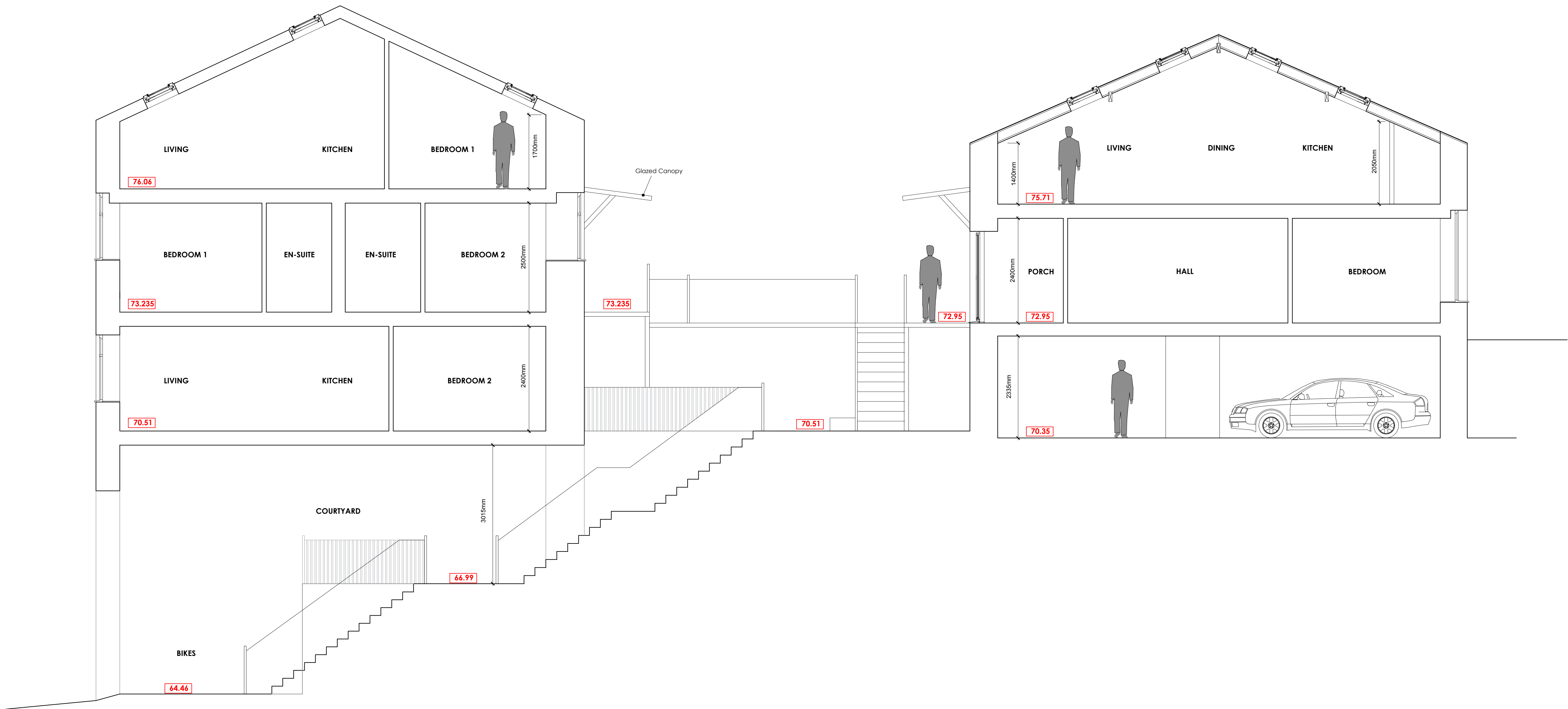
PROPOSED SECTION A-A SCALE 1:50
