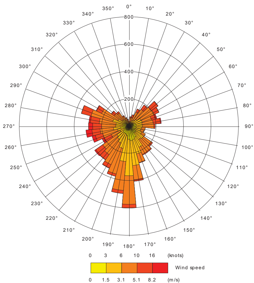
Figure C.2: 2018 Wind Rose for the Manchester Meteorological Station
