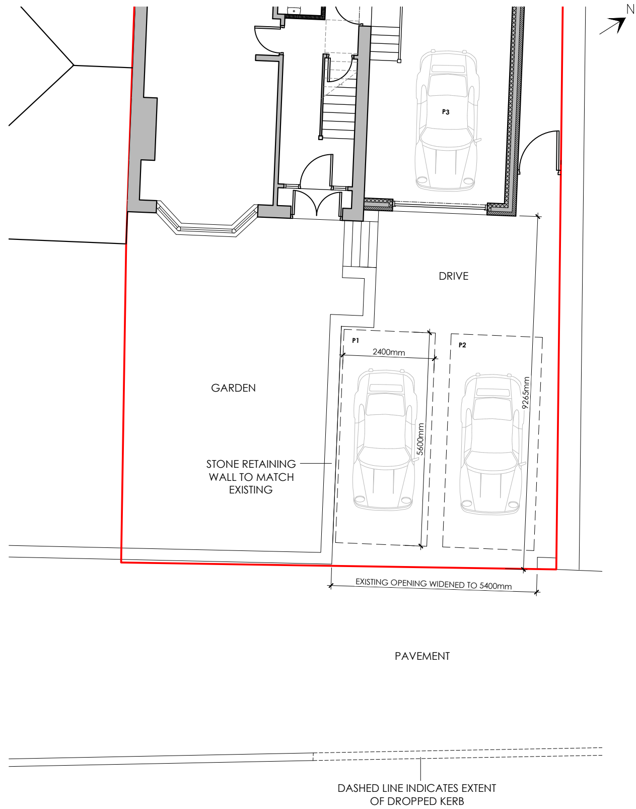
PROPOSED PART SITE PLAN Scale 1:100
