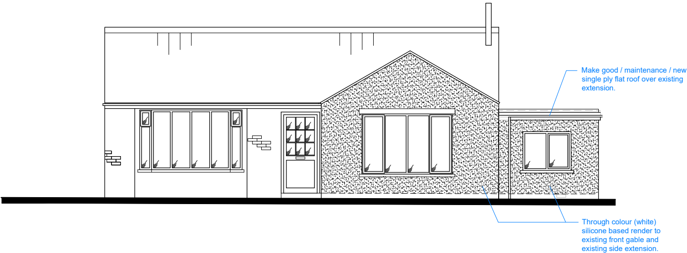
Sketch Front Elevation
