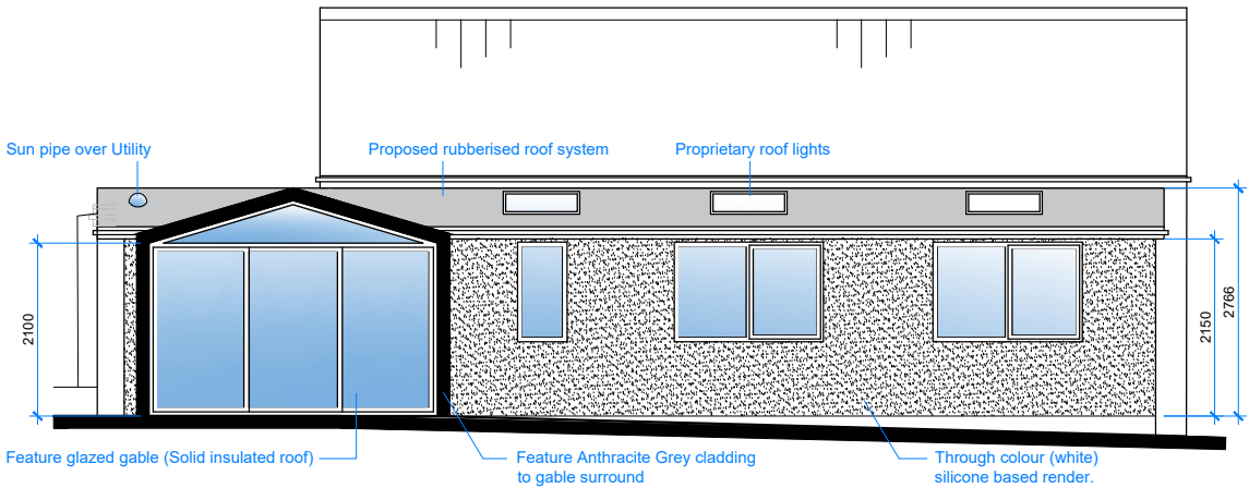
Sketch Rear Elevation
