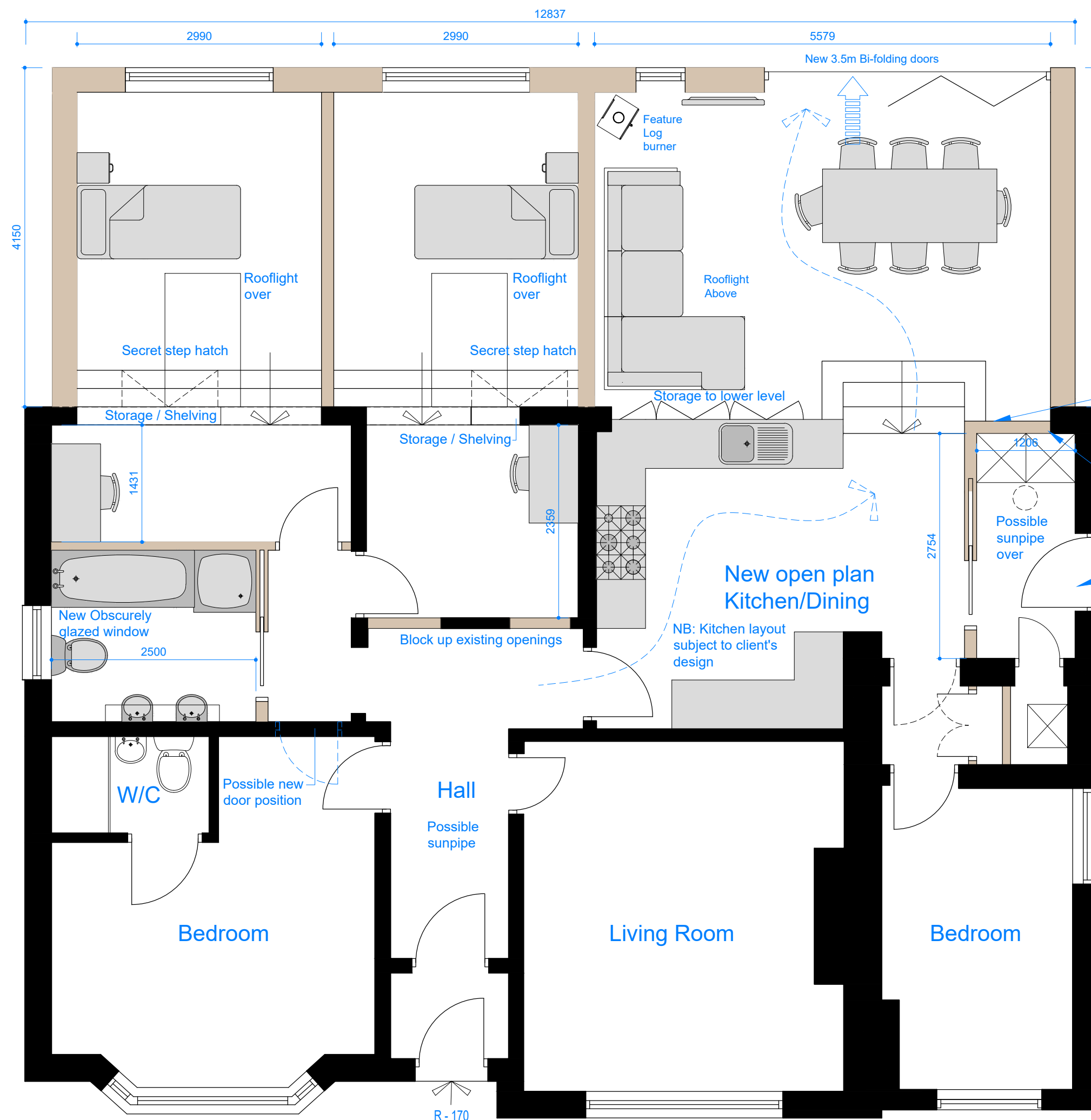
Sketch Pro. Ground Floor Plan
