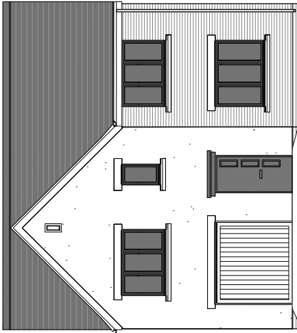
Front Elevation
