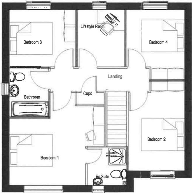
Revised First Floor
