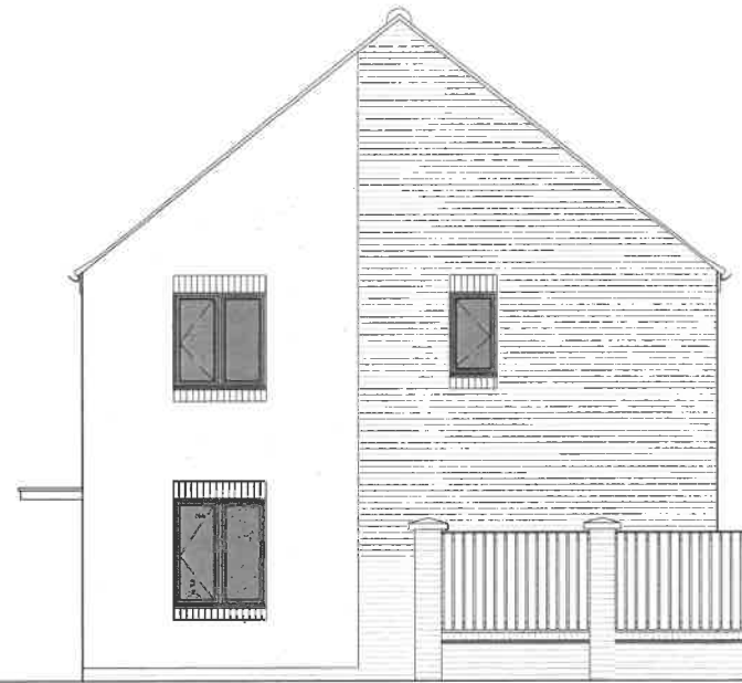
Side Elevation
