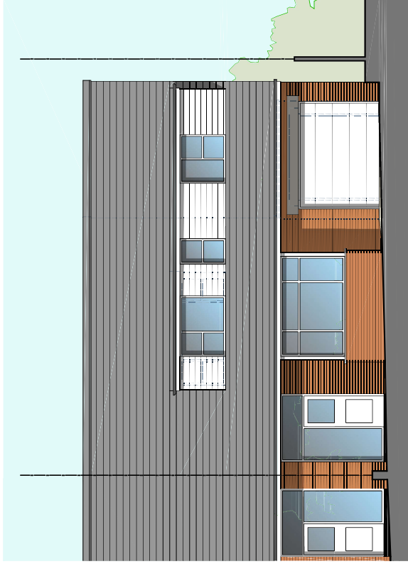
Front (South) Elevation
