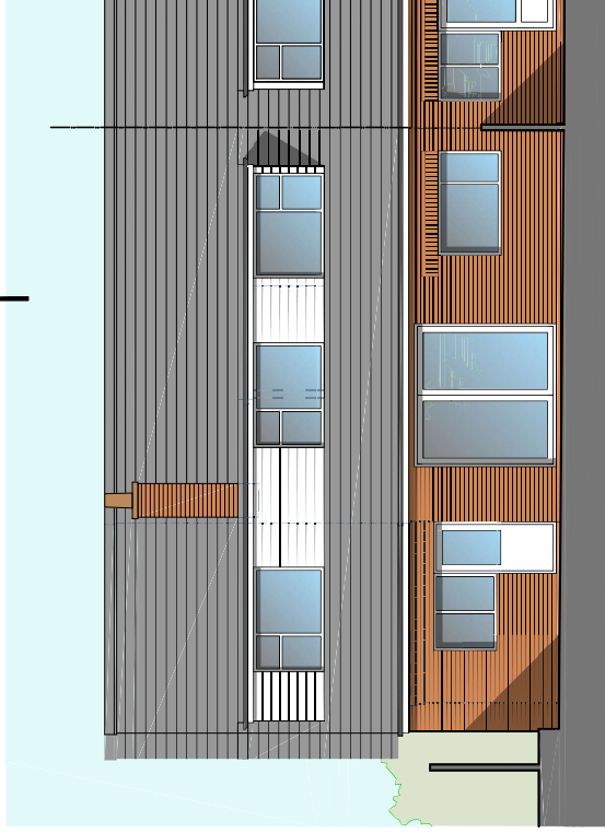
Rear (North) Elevation
