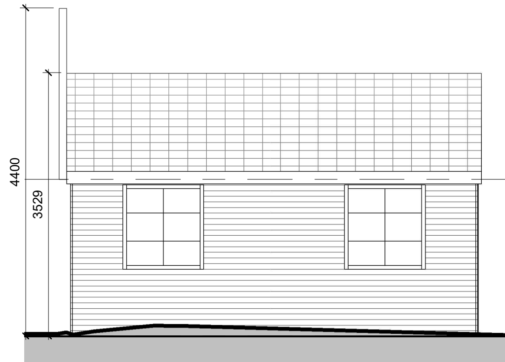
2 - Existing Side Elevation 1 : 50
