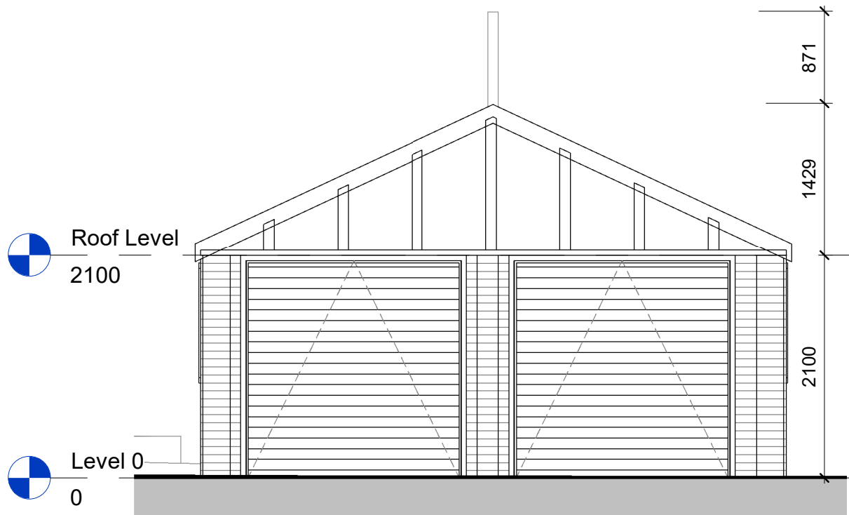
1 - Existing Front Elevation 1 : 50
