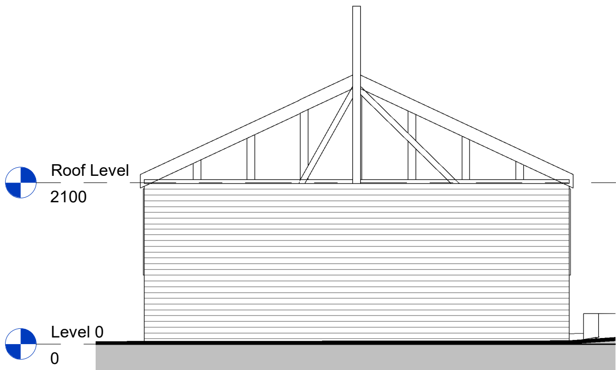
3 - Existing Rear Elevation 1 : 50
