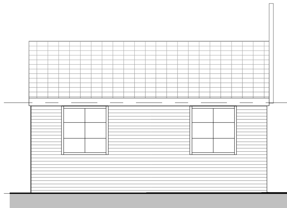
4 - Existing Side 2 Elevation 1 : 50
