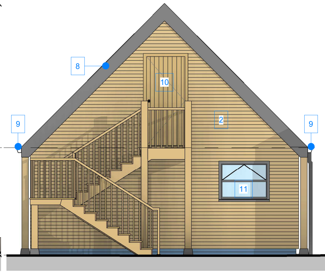
4 - Proposed Side 2 Elevation 1 : 50
