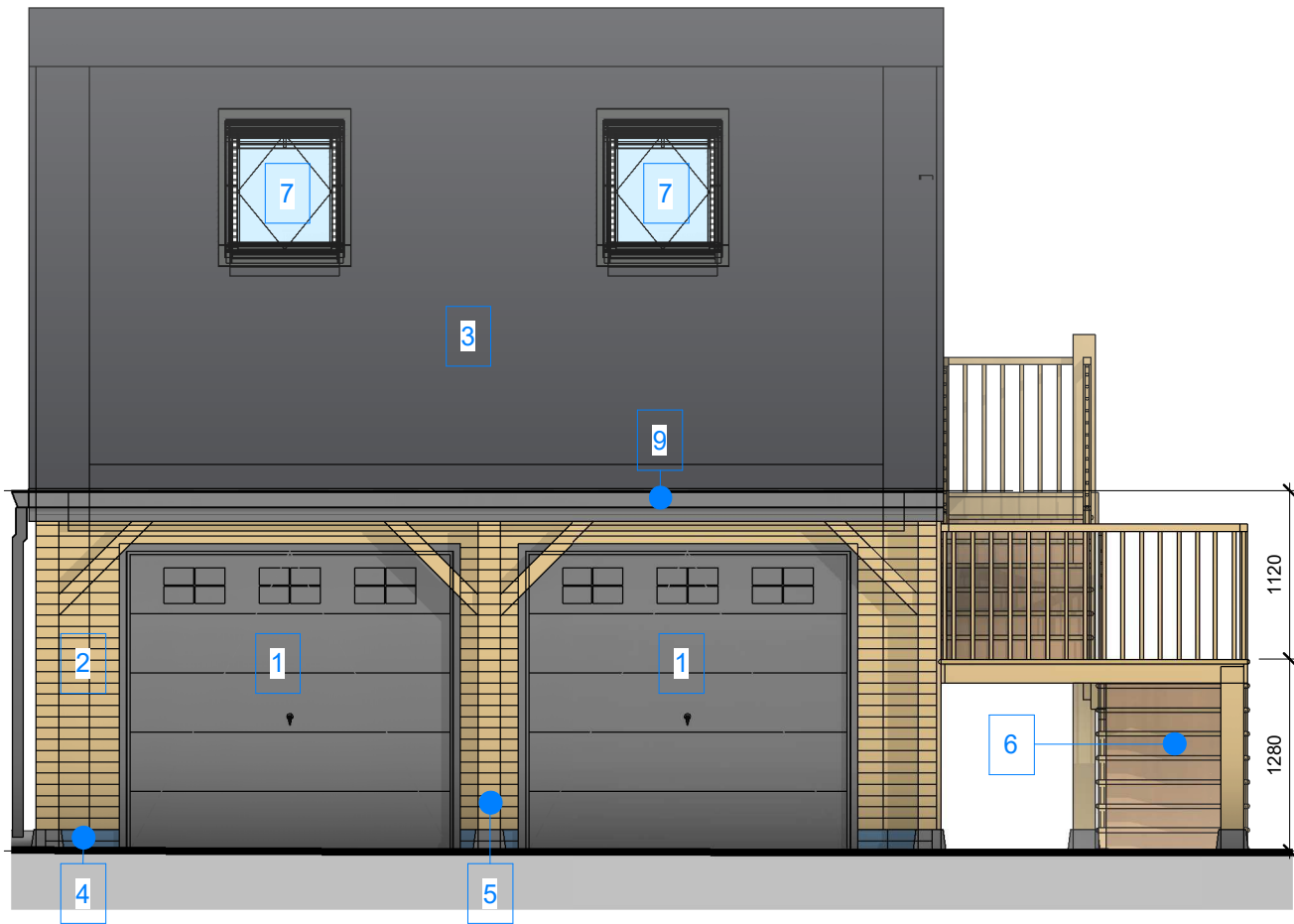
1 - Proposed Front Elevation 1 : 50
