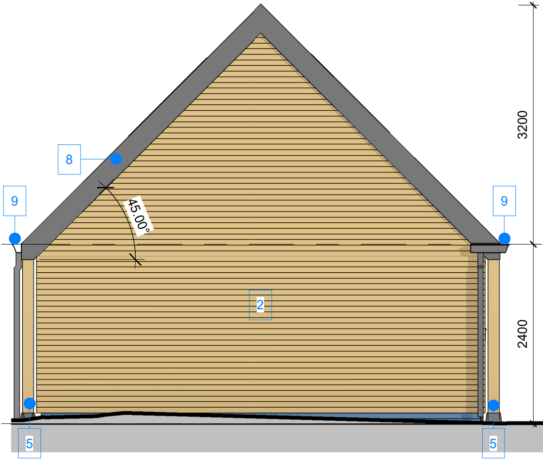
2 - Proposed Side Elevation 1 : 50
