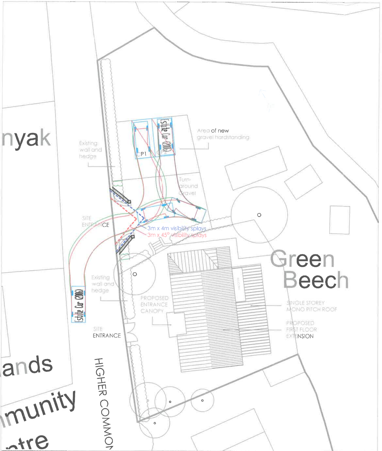
SITE LAYOUT PLAN (Visibility Splays & Turnaround)
