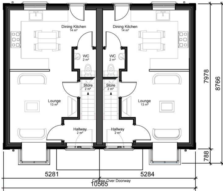
Proposed Ground Floor ( 35m ) 2
