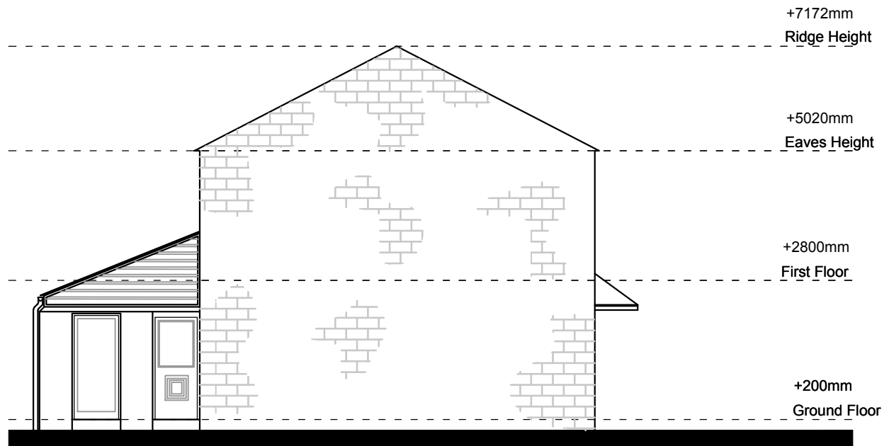
Side Elevation
