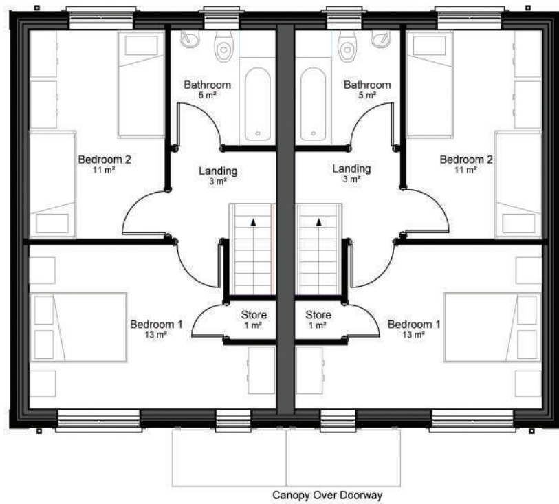
Proposed First Floor ( 35m ) 2
