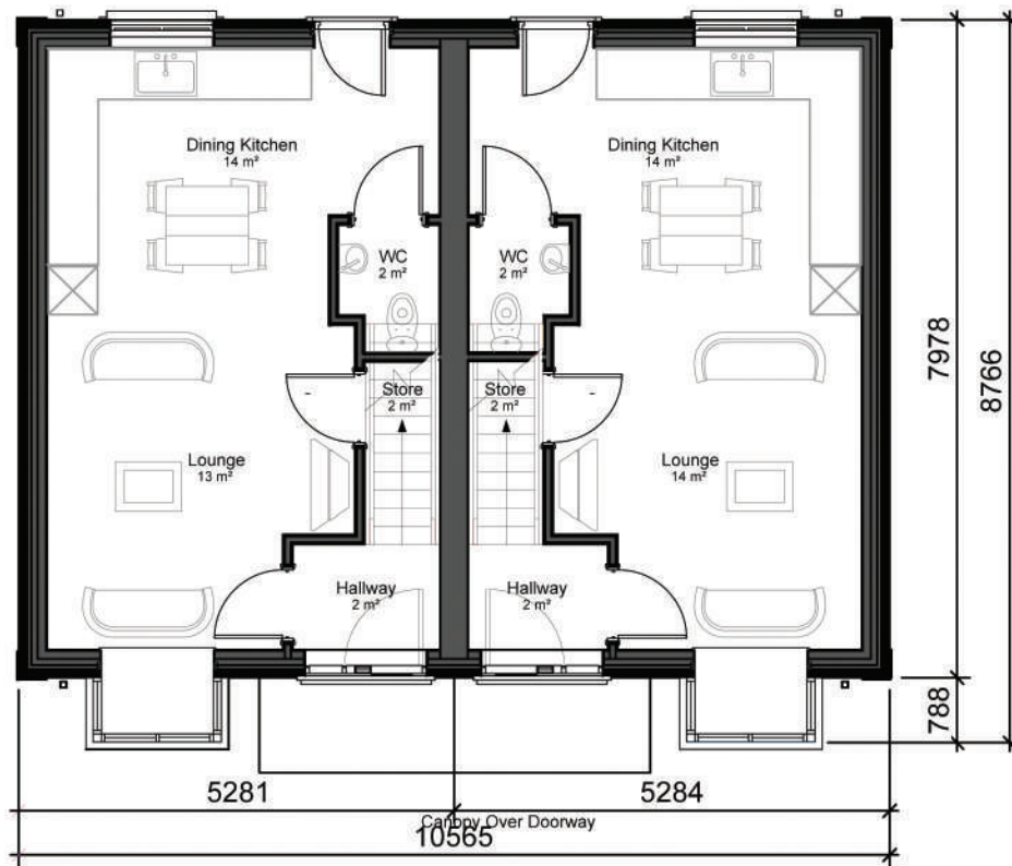
Proposed Ground Floor (35m)
