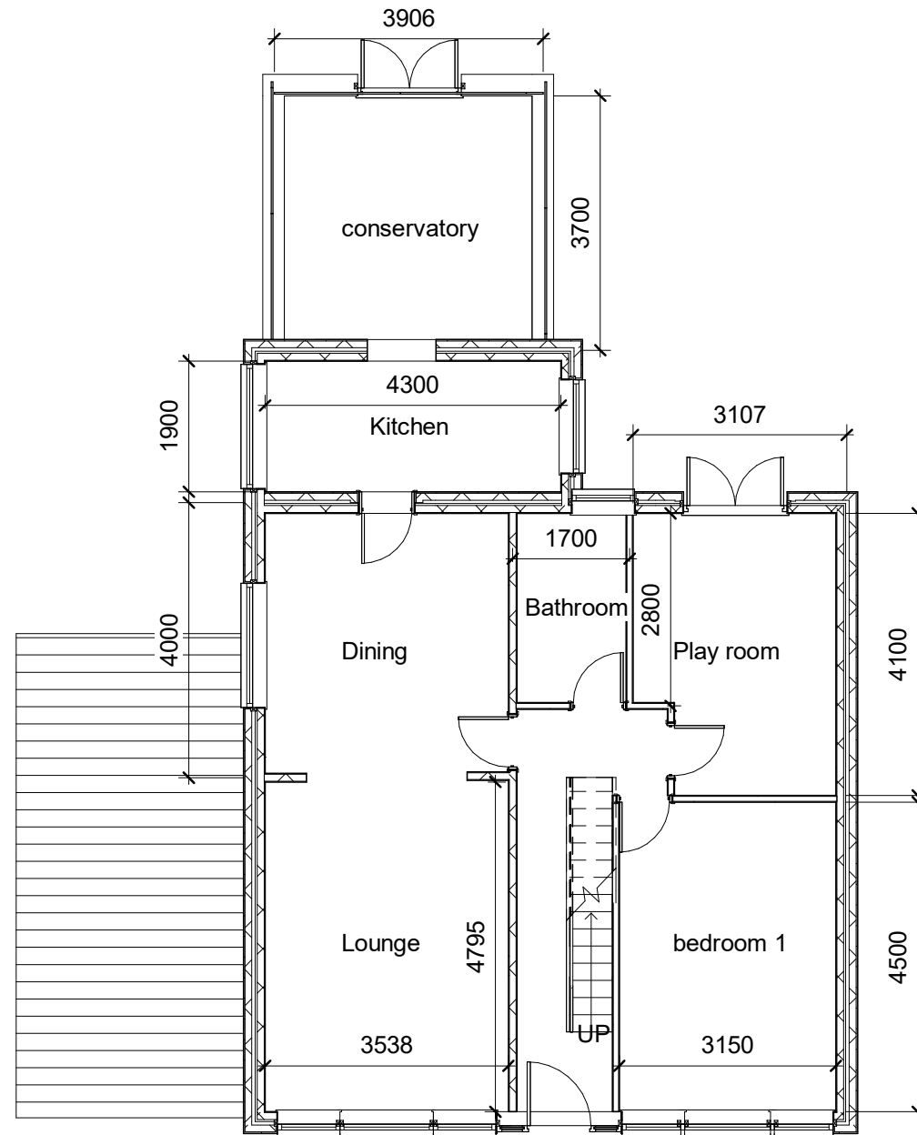
1 Ground floor 1 : 100
