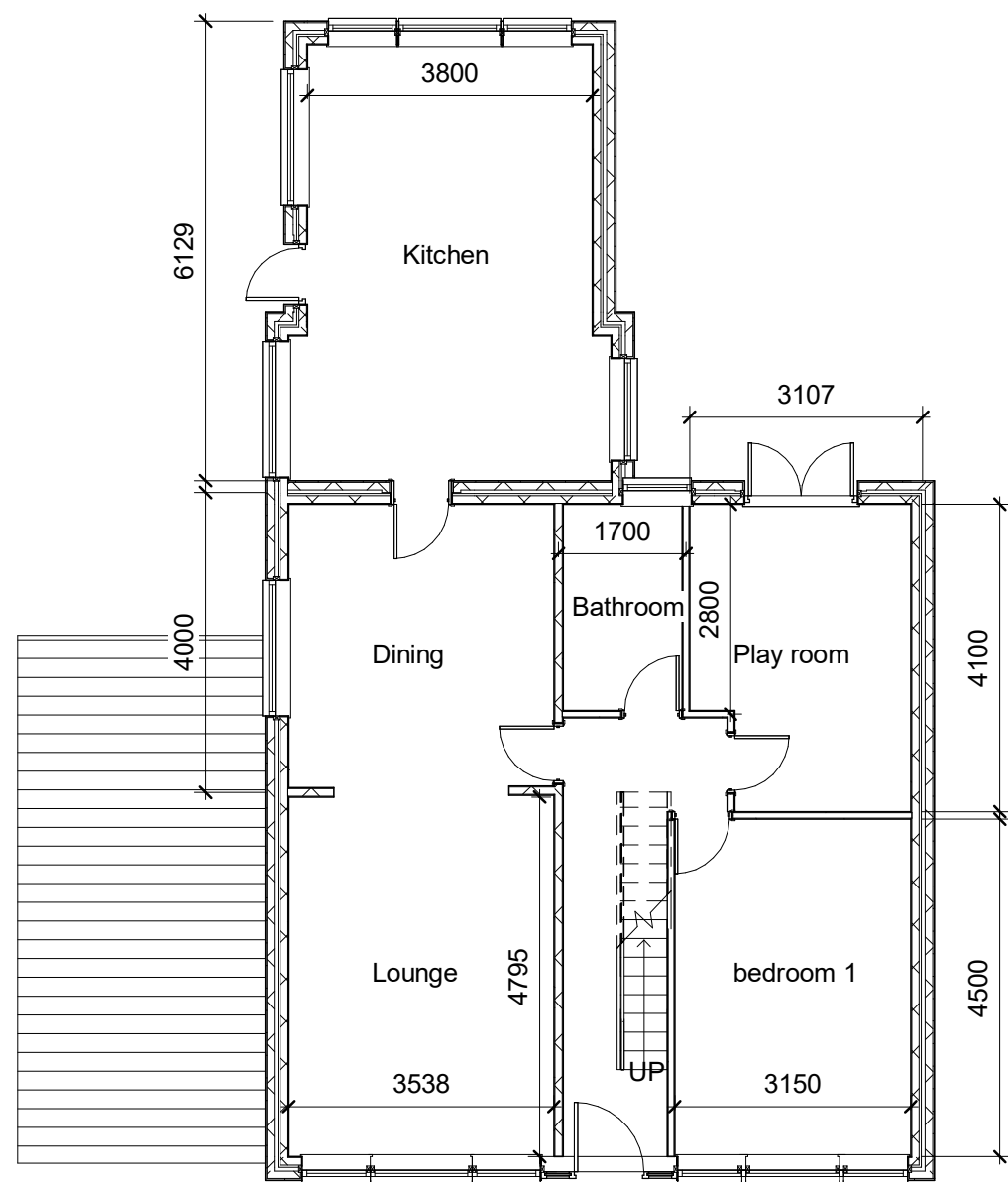
1 Ground floor 1 : 100
