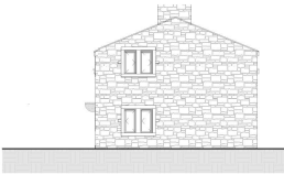
⑤ Proposed East 1 : 100
