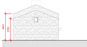
④ Proposed West 1 : 100
