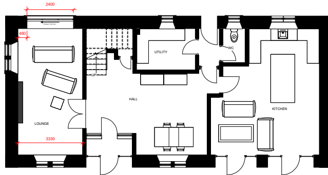
① Proposed Floor Plan 1 : 50
