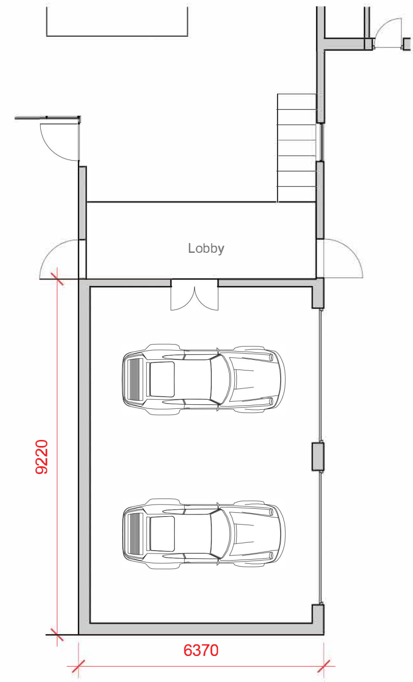
Proposed Garage Floor Plan 1 : 100
