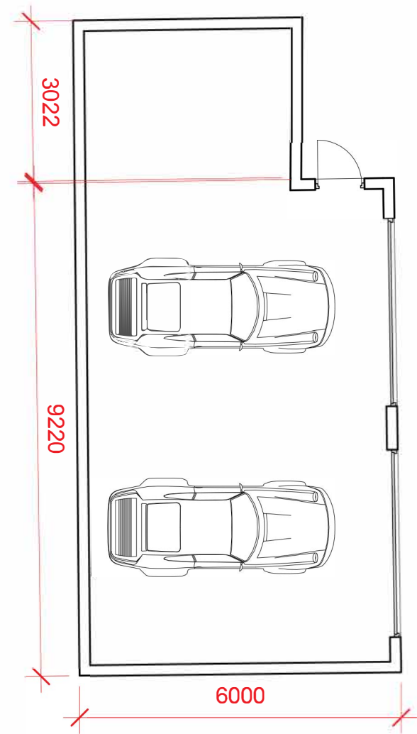
Existing Garage Floor Plan 1 : 100
