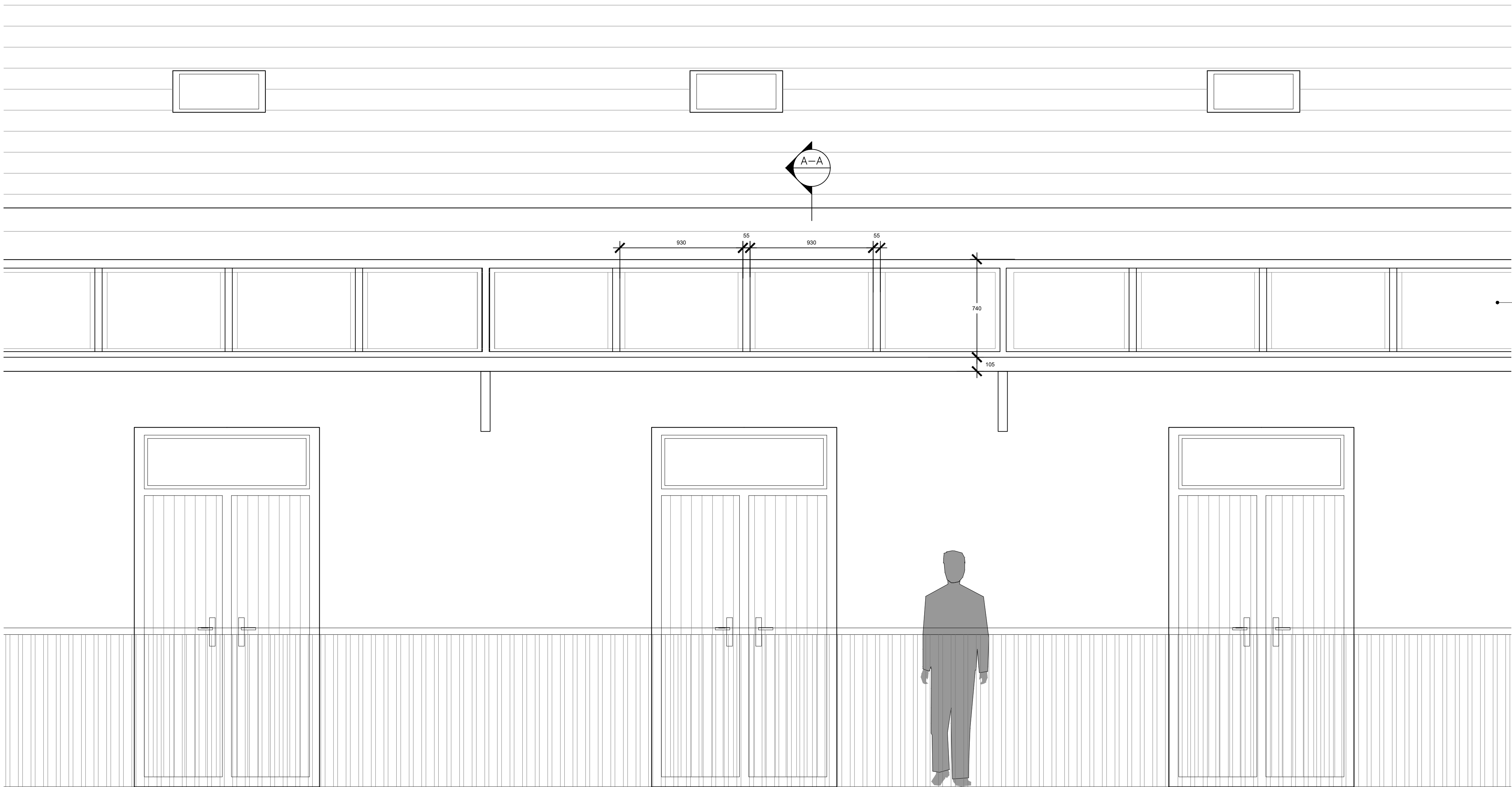
PART ELEVATION A SCALE 1:20
