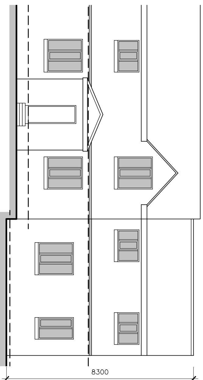
PROPOSED FRONT ELEVATION 1:100
