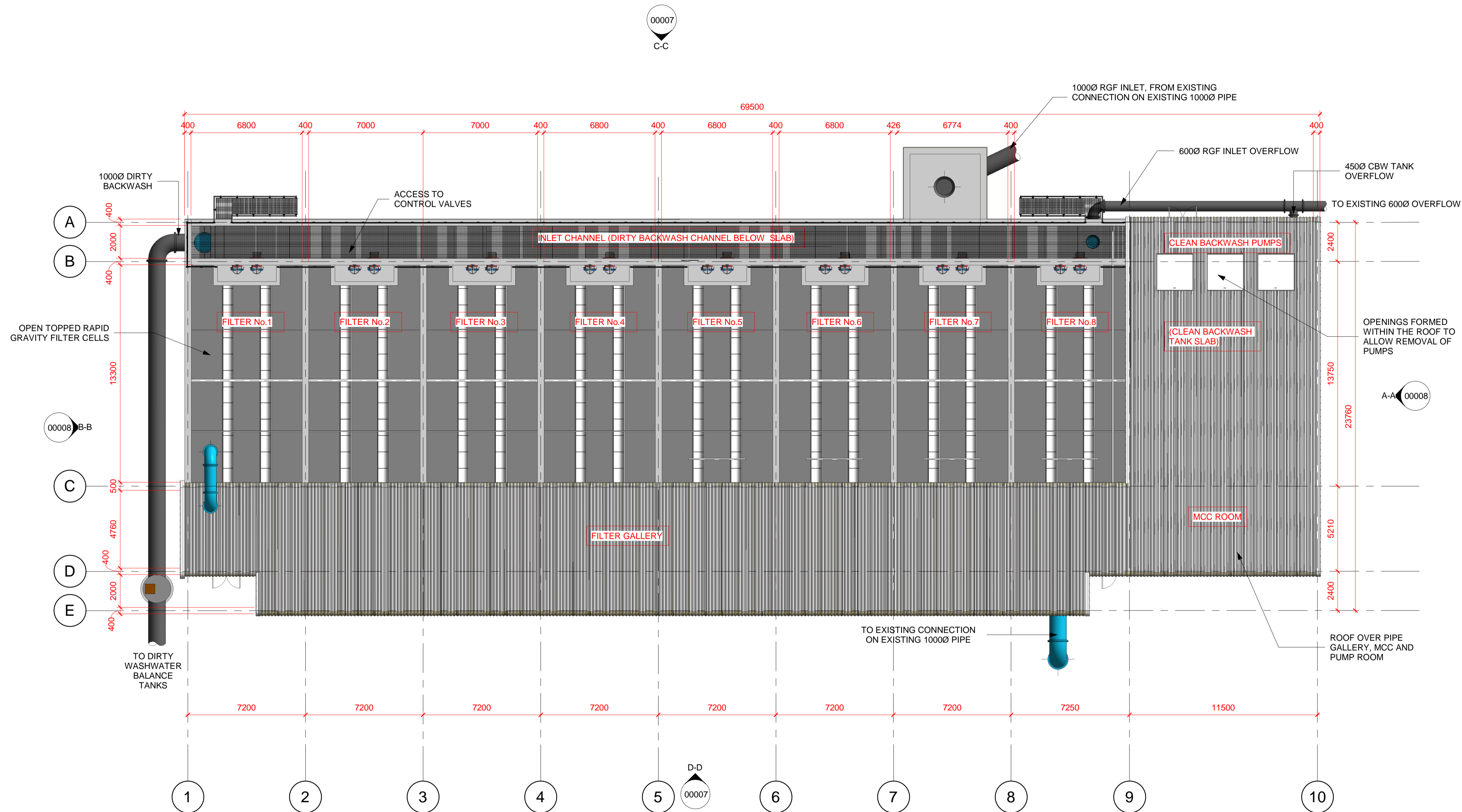
RAPID GRAVITY FILTERS PLAN 1 : 150
