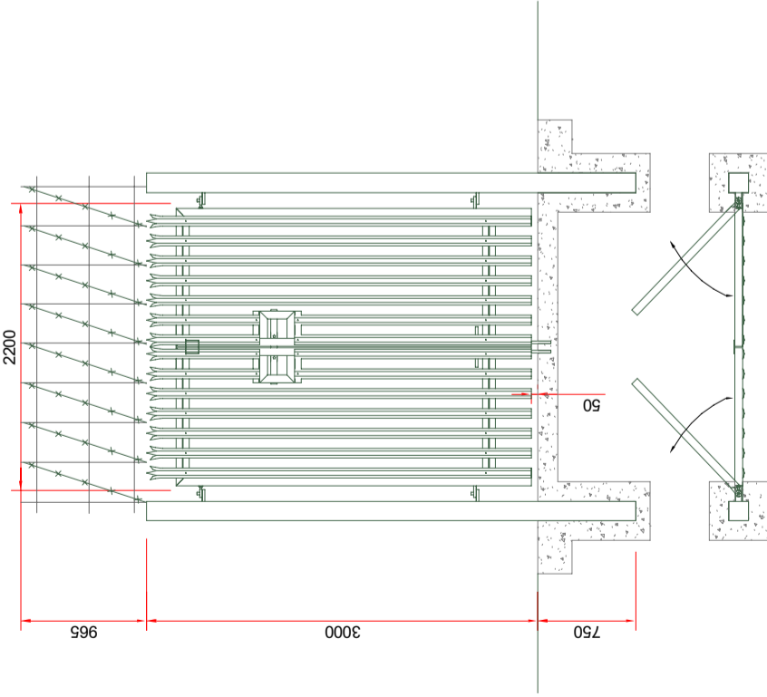
3M HIGH DOUBLE GATE WITH RAZOR WIRE TOP SCALE 1:50
