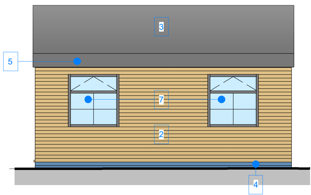
4 - Proposed Side 2 Elevation 1 : 50
