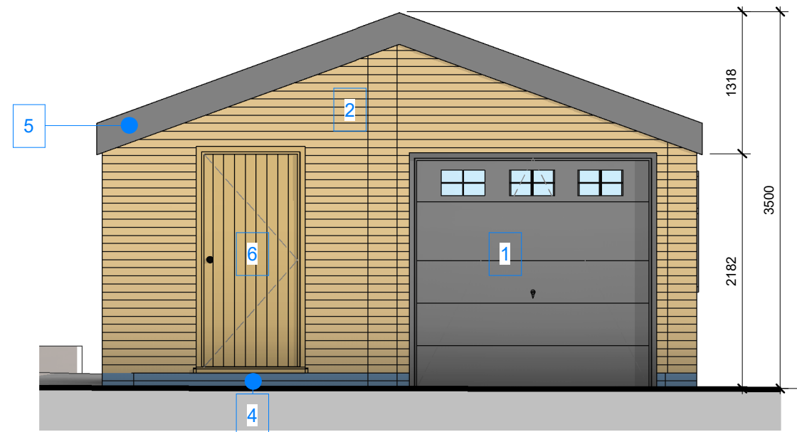
1 - Proposed Front Elevation 1 : 50
