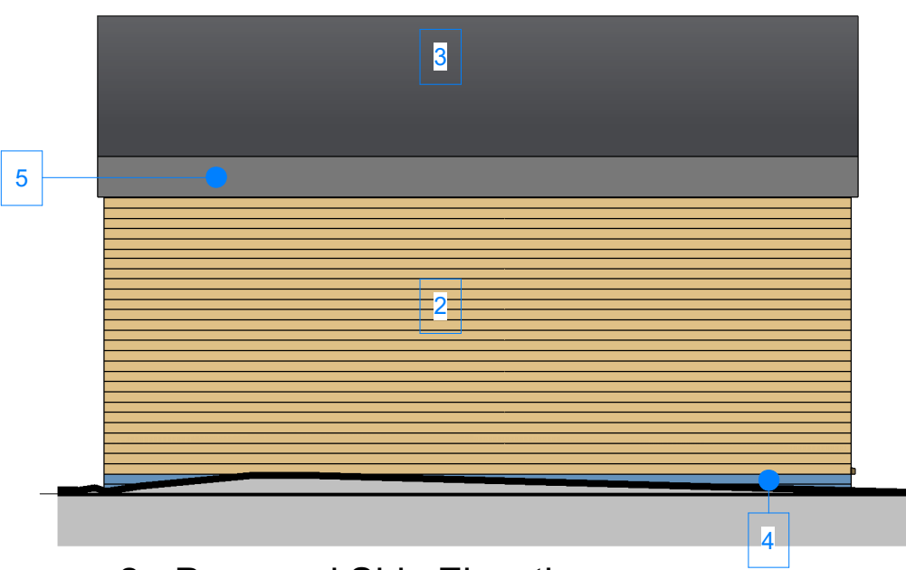
2 - Proposed Side Elevation 1 : 50
