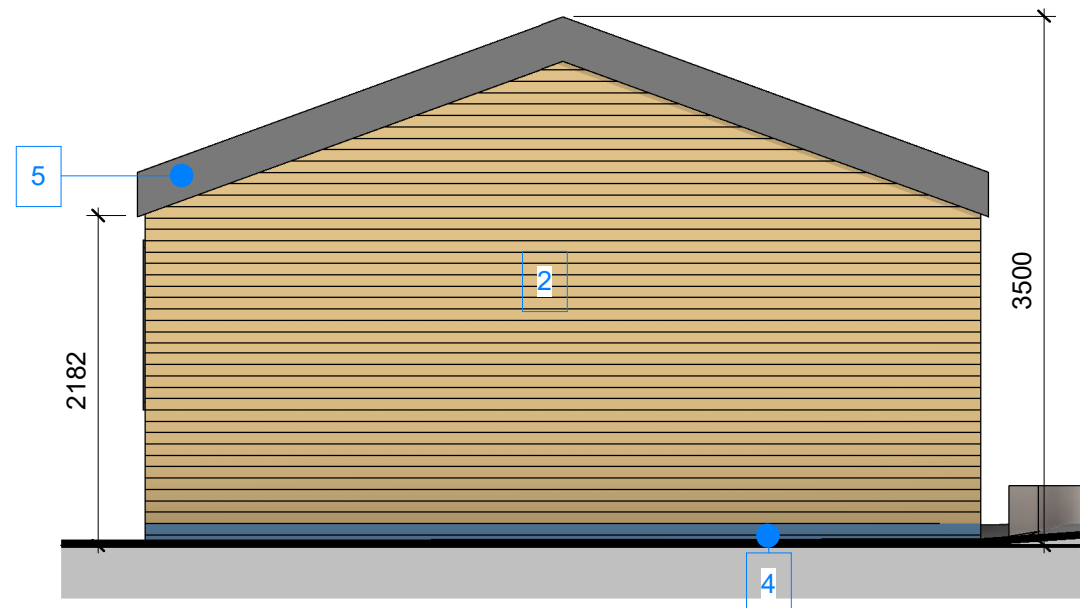
3 - Proposed Rear Elevation 1 : 50
